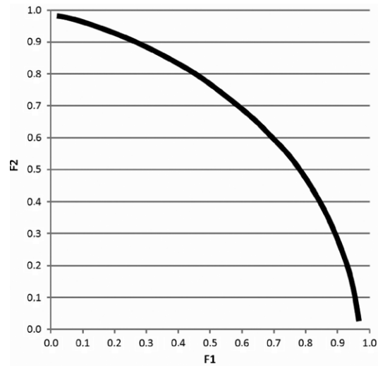
Fig. 3.2. Benchmark 1: reference Pareto front.
