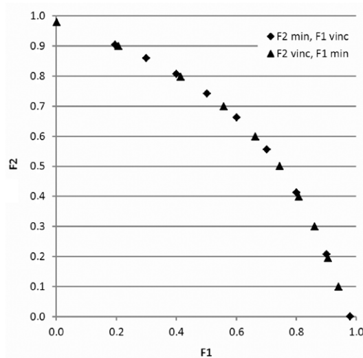
Fig. 3.6. Benchmark 1: ε-constraint method (iterations: 257).
