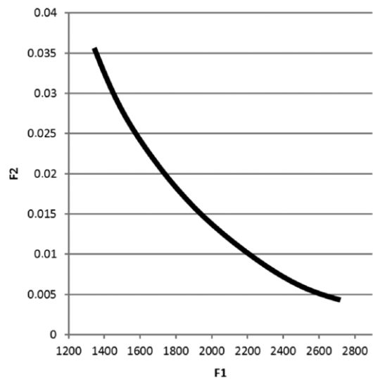
Fig. 3.13. Benchmark 3: reference Pareto front.
