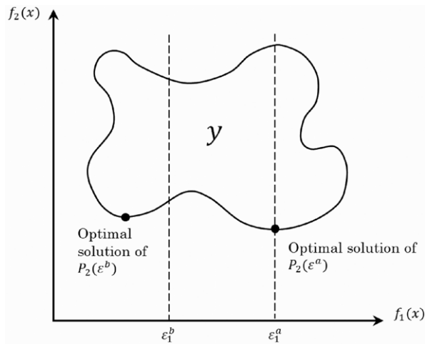
Fig. 2.2. Optimal solutions of \epsilon -constraint problems (1.26).
