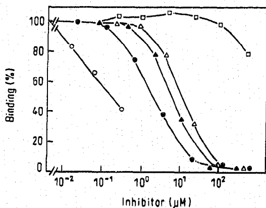
Fig. 2. Inhibition of binding of biotinylated integrin \alpha \text{IIb}\beta 3 to immobilized fibrinogen. Inhibitors used were fibrinogen (○), linear GRGDS (▲) and the cyclic peptides cRGDFV (●), cRGDFV (Δ) and cRADFV (□). Non-inhibited binding is set at 100%. Underlined residues correspond to D-isomers.
