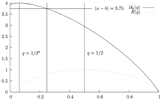
Fig. 3. the upper entropy for q in 4 bits
