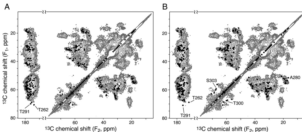
Fig. 7. Verification of structure models by 13 C– 13 C 2D data. The experimental spectrum (gray) was obtained with 10 ms DARR mixing [22]. Simulated spectra (black) for the trans -model (A) and cis -model (B) only consist of Cα–Cβ, Cα–CO, and Cβ–CO correlations, without other side chain carbons.
