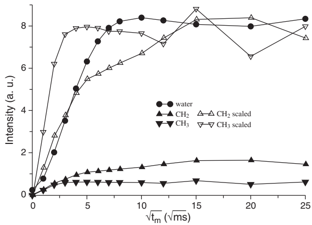
Fig. 4. Proton 1D spin diffusion data buildup curves as a function of mixing time. The CH 2 and CH 3 curves are also rescaled for easy comparison of buildup rates. The fast growing CH 3 curve (down triangle) indicates a close contact between protein and the phospholipid acyl chain terminals, meaning that this part is deeply buried inside the lipid bilayer. While the CH 2 group (up triangle) shows a clear biphasic behavior indicating that there are two types of interactions with CH 2 groups from the protein, possibly the one buried inside the bilayer and the one in the cytosol part. The experiment was performed at 45 °C and data points were corrected for T 1 relaxation.
