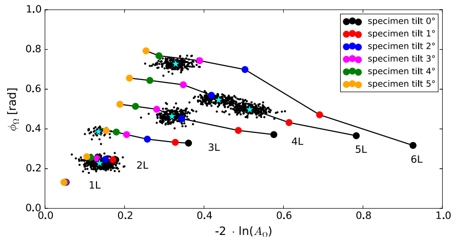
Fig. 7. Plot of phase shift \phi_0 vs -2\ln(A_0) extracted from experimental data by averaging in Voronoi cells corresponding to unit cells and simulated wavefunctions. The experimental data are in well-separated clouds and can therefore be assigned uniquely to different numbers of WSe 2 layers by taking into account specimen tilt angles of a few degrees. The simulated values are displayed by colored circles. Lines connect the points corresponding to the same thickness, labeled by number of layers (1L to 6L). The experimental data are plotted in the form of small black dots and the cyan colored stars display the center of mass of each cloud.
