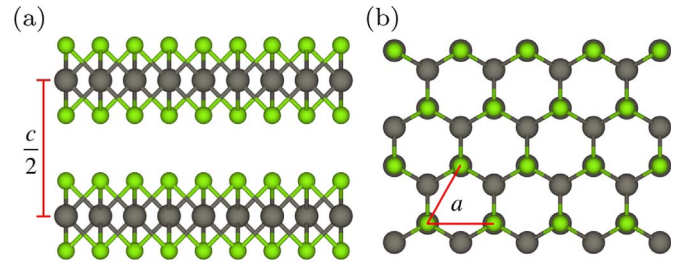
Fig. 1. Crystallographic structure of 2H- \text{WSe}_2 with the lattice parameters a = 3.28 \text{ \AA} and c = 12.96 \text{ \AA} [14]. Green spheres represent Se atoms, while gray spheres represent W atoms. (a) View of the \text{WSe}_2 lattice along [-120] , illustrating its layered structure. (b) View of the \text{WSe}_2 lattice along [001] . The crystal structures are visualized using Vesta software [15]. (For interpretation of the references to color in this figure legend, the reader is referred to the web version of this article.)
