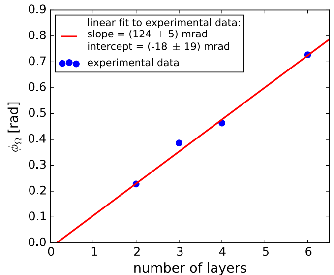
Fig. B1. Linear fit to experimental phase measurements plotted as a function of specimen thickness to obtain the average phase shift per \text{WSe}_2 layer. The fitted parameters are shown in the legend as a slope and intercept. The error in each point, determined from the standard error in the mean, is too small to be visualized.
