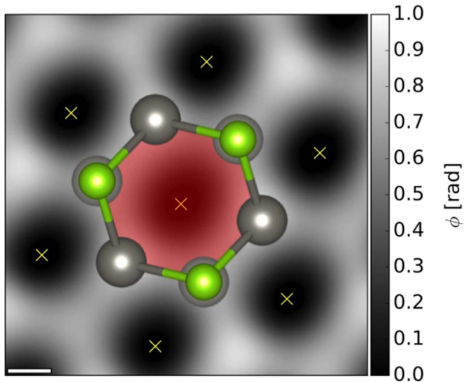
Fig. 3. Schematic diagram illustrating the setup of Voronoi tessellation on a phase image of \text{WSe}_2 . Green and gray spheres represent Se and W atoms, respectively. The yellow crosses show the positions of local minima in phase. An example of a Voronoi cell corresponding to the central minimum is marked by a red hexagon. The scale bar is 1 Å. (For interpretation of the references to color in this figure legend, the reader is referred to the web version of this article.)
