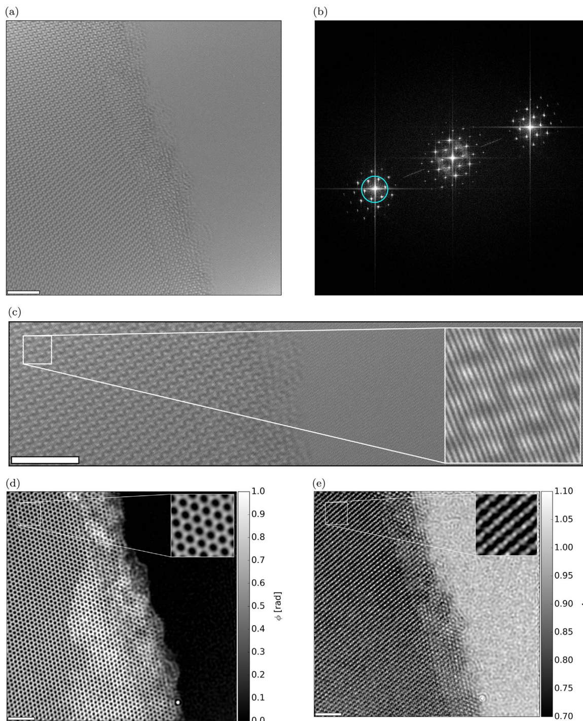
Fig. 4. (a) Off-axis electron hologram of a few-layer-thick \text{WSe}_2 crystal recorded at 80 kV, with a vacuum area on the right side. (b) Fourier transform of the hologram, with a circular mask of semi-angle 15 mrad marked around one of the sidebands by a circle. (c) Enlarged view of the top quarter of the hologram shown in Fig. 4a. The holographic fringes and their modulation due to the interaction with the atomic structure are visualized in the inset, which shows a small area at higher magnification. (d) Phase and (e) amplitude of the electron wavefunction reconstructed using the 15 mrad mask shown in Fig. 4b. The insets show magnified images of the marked areas. All scale bars are 2 nm.
