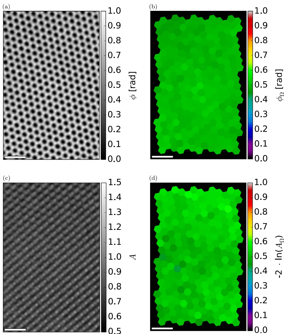
Fig. 5. (a) Phase \phi and (c) amplitude A images of the same region of a clean area of few-layer-thick \text{WSe}_2 taken from the top left part of Fig. 4. (b) Phase \phi_{\Omega} and (d) -2 \ln(A_{\Omega}) after averaging within the area of each Voronoi cell \Omega constructed from the phase image in (a). The scale bars are 1 nm.
