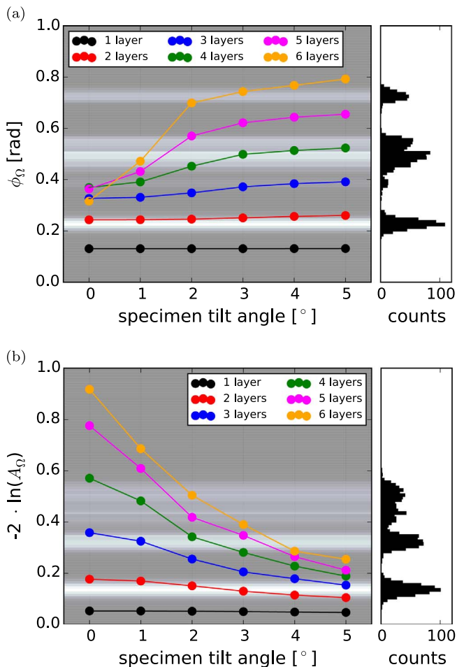
Fig. 6. Values of (a) \phi_0 and (b) -2\ln(A_0) obtained from simulations, plotted as a function of specimen tilt angle for different numbers of WSe 2 layers (i.e., different values of specimen thickness). The background in each plot shows a histogram (binning: 0.01 rad and 0.01, respectively) of corresponding experimentally measured values, where a bright color corresponds to a high number of counts and a dark color to a low number of counts. The experimental values are averaged over different specimen tilt angles. The histograms are shown more conventionally on the right side of each graph. (For interpretation of the references to color in this figure legend, the reader is referred to the web version of this article.)
