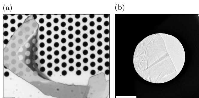
Fig. 2. (a) Light-optical micrograph and (b) low magnification TEM image of a WSe 2 flake transferred onto a Au-coated holey SiN membrane. The holes in the SiN membrane are 2.5 μm in diameter. The scale bars are (a) 5 μm and (b) 1 μm.
