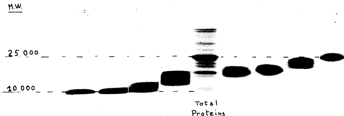
Fig. 2. Analytical electrophoresis of different fractions obtained after preparative electrophoresis in the mol. wt. range from 10 000 to 25 000.
