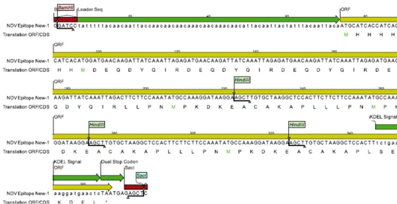
Fig. 1. Gene construct including F and HN epitopes together with needed sequences for expression in tobacco.
