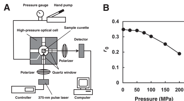
Fig. 2. Construction of a system employing HP-TRFAM. (A) A high-pressure optical cell with quartz windows capable of applying hydrostatic pressure was mounted in a FluoroCube designed to perform TCSPC with a polarizing device and a 375-nm laser diode operated with a pulse frequency of 1 MHz. (B) A calibration curve was derived by measuring r_0 values for 1 \mu M DPH in mineral oil under various hydrostatic pressures to correct the strain birefringence of the quartz windows caused by high pressure. Data represent mean \pm SD from three independent experiments. Error bars are shown within the symbols.
