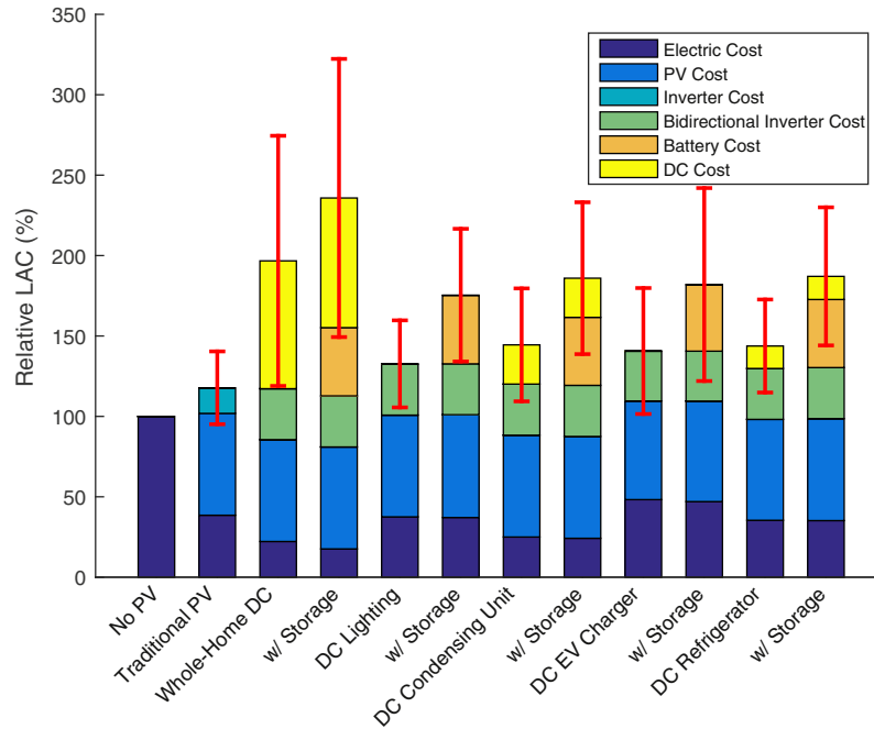
Fig. 3. Levelized annual costs for the systems shown in Fig. 1(a) through Fig. 1(g). Results are shown as a percentage of a traditional (AC) home with no PV generation's annual electric bill. Discount rate was varied from 5% to 10%. Bars show the mean result for each simulation. Error bars show plus or minus one standard deviation from the mean.
