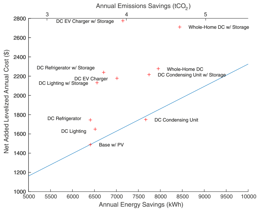
Fig. 4. Average cost-effectiveness of savings associated with each simulated DC home configuration. Average annual energy and emissions savings are shown on the x-axes. The net cost added to a traditional AC home's LAC by implementing each scenario is shown on the y-axis. This cost includes the cost of the PV system in every configuration. The blue line shows the cost-effectiveness (in $/kWh saved and $/tCO 2 saved) of installing a solar PV array without considering any utility incentives. All values shown are the mean of all homes in each sample. (For interpretation of the references to color in this figure legend, the reader is referred to the web version of this article.)
