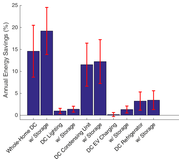
Fig. 2. Annual energy savings for simulated direct-DC systems. Savings are reported as a percentage of baseline energy consumption of traditional AC homes. Simulation results correspond to the systems shown in Fig. 1(c) through Fig. 1(g). Error bars show plus or minus one standard deviation from the mean.
