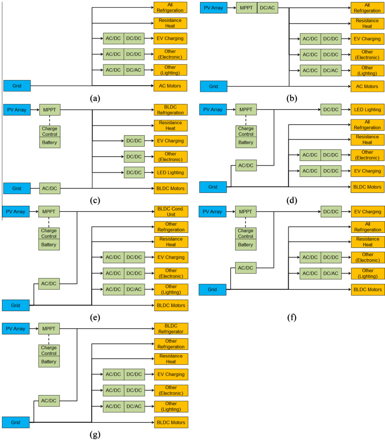
Fig. 1. Schematic diagrams of simulated home configurations: (a) traditional home with AC distribution, without PV (b) traditional home with AC distribution and net-metered solar PV (c) home with DC distribution to all loads and net-metered PV with grid-rectified backup (d) home with DC distribution to a lighting circuit and net-metered PV with grid-rectified backup (e) home with DC distribution to a condensing unit and net-metered PV with grid-rectified backup (f) home with DC distribution to a PEV charger and net-metered PV with grid-rectified backup (g) home with DC distribution to a refrigerator and net-metered PV with grid-rectified backup.
