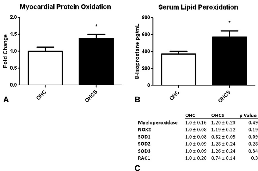
FIGURE 3. Oxidative stress profile. A, Myocardial protein oxidation showing significantly increased protein oxidation in oral hypercaloric/hypercholesterolemic diet plus 1.5 mg/kg atorvastatin daily (OHCS) compared with oral hypercaloric/hypercholesterolemic diet (OHC) groups. B, Serum lipid peroxidation. Significantly increased lipid peroxidation was seen in OHCS group compared with OHC group. C, Western blot analysis of oxidative stress protein expression showing no difference in expression of proteins involved in oxidative stress. * P < .05 . AMPK, Adenosine monophosphate kinase; eNOS, endothelial nitric oxide synthase; pAkt, phosphorylated Akt; pAMPK, phosphorylated AMPK; peNOS, phosphorylated eNOS; VEGF, vascular endothelial growth factor; VEGFR2, VEGF receptor 2.
