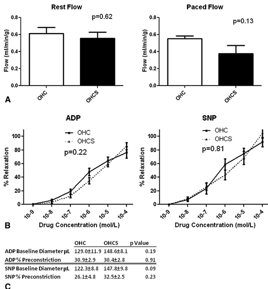
FIGURE 1. Myocardial perfusion and coronary microvessel reactivity. A, Myocardial perfusion at rest and with demand pacing. No difference was seen in myocardial perfusion at rest or during demand pacing at 160 beats/min. B, Microvessel reactivity. No difference was seen in microvessel reactivity to endothelium-dependent (adenosine diphosphate [ADP]) or endothelium-independent (sodium nitroprusside [SNP]) vasodilators in oral hypercaloric/hypercholesterolemic diet (OHC) and oral hypercaloric/hypercholesterolemic diet plus 1.5 mg/kg atorvastatin daily (OHCS) groups. C, Baseline microvessel diameter and percentage of precontraction. No difference was seen in baseline diameter or percentage of precontraction in ADP- or SNP-treated microvessels.
