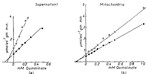
Fig. 1. Reciprocal velocity against inhibitor concentration plots for quinolinate inhibition of (a) supernatant and (b) mitochondrial PEPCK. Experiments were conducted using increasing concentrations of quinolinate at oxaloacetate concentrations of (a) 17.6 \mu\text{M} ( \bullet - \bullet ) and 9.6 \mu\text{M} ( \circ - \circ ), and (b) 19.2 \mu\text{M} ( \bullet - \bullet ) and 10.7 \mu\text{M} ( \circ - \circ ). ITP was present at 5 mM and \text{Mn}^{++} at 1 mM temperature of 37°C. The velocity of the PEPCK reaction was measured in the direction of PEP synthesis as described in the methods section.
