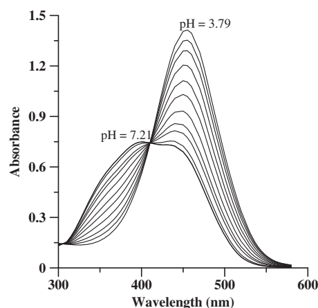
Figure 2 Spectra of chrysoidine 5.6 \times 10^{-5} M, path length 1 cm, and variable pH from 3.79 to 7.21.
