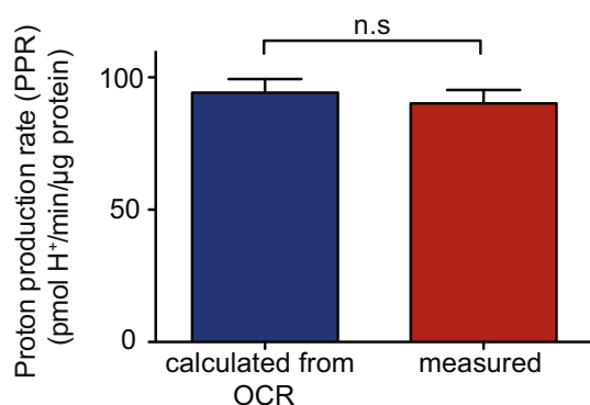
Fig. 3. Proton production rates calculated from oxygen consumption rate and measured using calibrated pH changes. The calculated proton production rate was determined from the rotenone-sensitive oxygen consumption rate in Fig. 1B (see Materials and Methods). The measured proton production rate was taken from Fig. 2D. Data are means ± SEM of n = 6 independent biological replicates. n.s.: p = 0.58 , two-tailed paired Student's t -test.
