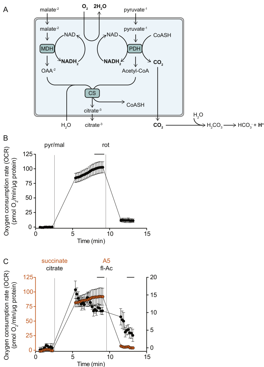
Fig. 1. Reactions of the model \text{CO}_2 -generating system. (A) Metabolic reactions involved in \text{CO}_2 generation by isolated rat skeletal muscle mitochondria respiring on pyruvate plus malate and generating citrate. MDH, malate dehydrogenase; PDH, pyruvate dehydrogenase; CS, citrate synthase. (B) Oxygen consumption rate of mitochondria in the presence of 4 \mu\text{M} FCCP, 2.5 \mu\text{g}/\text{mL} oligomycin, 5 mM dichloroacetate, 5 mM aminooxyacetate, 5 mM fluoroacetate, and 2 \mu\text{M} atpenin A5 measured in the Seahorse XF24. 10 mM pyruvate plus 2 mM malate and 1 \mu\text{M} rotenone were added as indicated. Data are means \pm SEM of n = 6 independent biological replicates. (C) Efficacy of fluoroacetate and atpenin A5. Respiration caused by addition of citrate (black axis and symbols) or succinate (red axis and symbols) was inhibited by subsequent addition of fluoroacetate or atpenin A5, respectively. Data are means \pm SEM of n = 3 independent biological replicates. Horizontal bars: the mean of this range was used for subsequent calculations.
