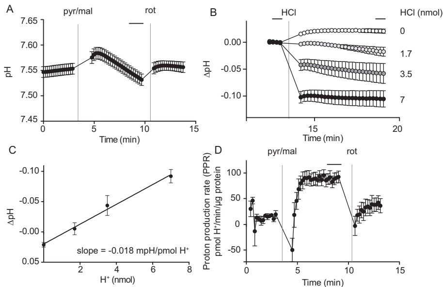
Fig. 2. Changes in pH and proton production rate caused by CO 2 production in the model system. (A) pH of the medium measured in the same experiments as Fig. 1B. Horizontal bar: pH values used to calculate acidification rate. (B) Acid calibration of buffering power. Different amounts of HCl were added from port C where indicated, in continuations of the experiment in A. Data were normalized to the mean of the last three points measured before acid addition. Values for HCl added are given relative to the 7 μL measuring volume, i.e., 1 mM added HCl corresponded to 7 nmol HCl in the measuring volume. Horizontal bars indicate initial and final data used to calculate the changes in pH. (C) Change in pH as a function of H + added to the 7 μL measuring volume (data from B). The slope is the buffering power, used to calibrate the rates of pH change shown in (A). (D) Proton production rate (PPR) calculated using the pH trace (A), calibration (B, C) and mitochondrial protein loaded per well. Horizontal bar: values used for proton production rate in Fig. 3. Data are means ± SEM of n = 6 independent biological replicates.
