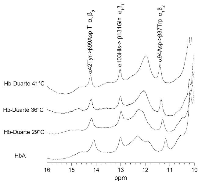
FIGURE 7 Hyperfine shifted and exchangeable proton resonances of HbA and Hb Duarte in the deoxy form collected at several temperatures.
