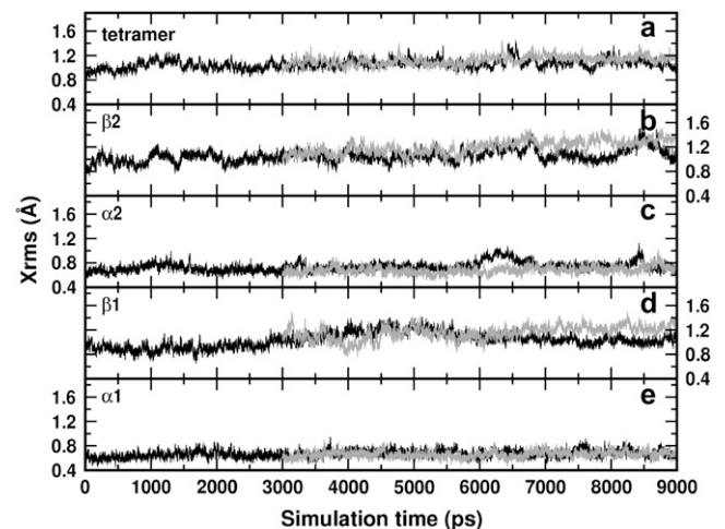
FIGURE 10 Xrms of deoxy HbA ( black curves ) and mutated ( gray curves ) hemoglobins: (a) tetramer, (b)–(e) \beta 2 , \alpha 2 , \beta 1 , and \alpha 1 chains, respectively.
