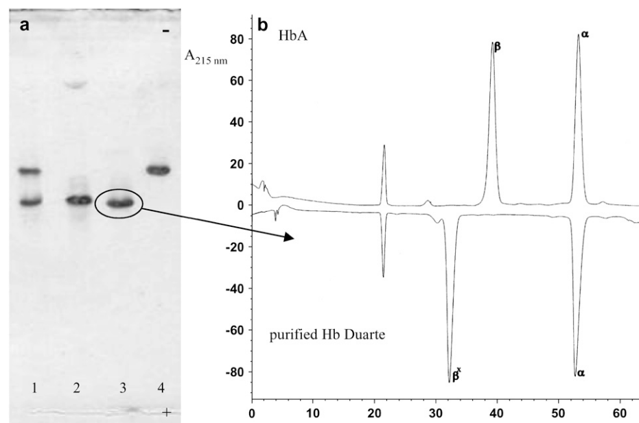
FIGURE 2 (a) IEF of total hemolysate (line 1), HbA (line 2), and Hb components purified by IEC (lines 3 and 4); (b) RP-HPLC of the globin chains of HbA and purified Hb Duarte.
