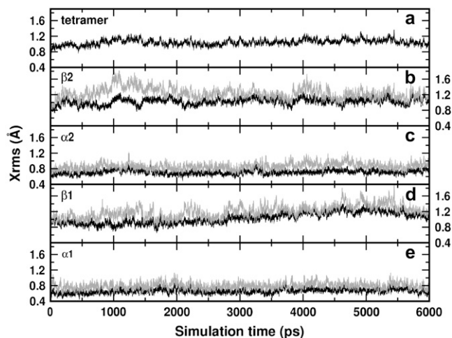
FIGURE 9 Xrms of deoxy HbA: (a) tetramer, (b)–(e) \beta 2 , \alpha 2 , \beta 1 , and \alpha 1 chains, respectively. The black curves refer to the deviations, the gray curves to the absolute deviations.
