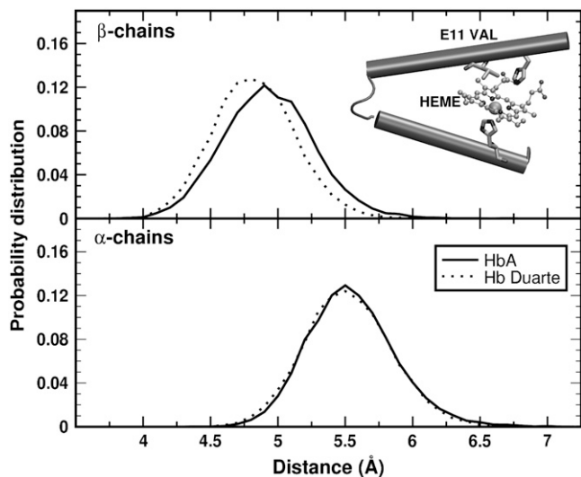
FIGURE 14 Distribution of the distance CG(1-2)(ValE11)-Fe (see inset) in the \beta - (upper panel) and \alpha - (lower panel) chains for deoxy HbA (solid lines) and deoxy Hb Duarte (dashed lines) during the simulation.
