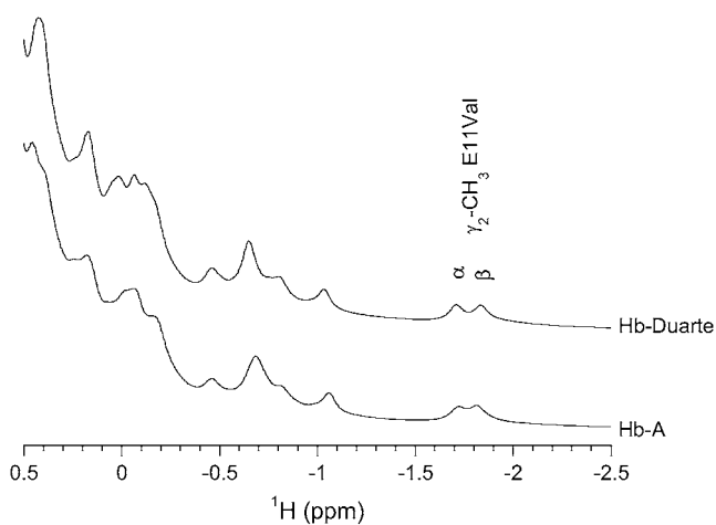
FIGURE 4 Downfield ring current-shifted resonances of HbA and Hb Duarte in the CO form.
