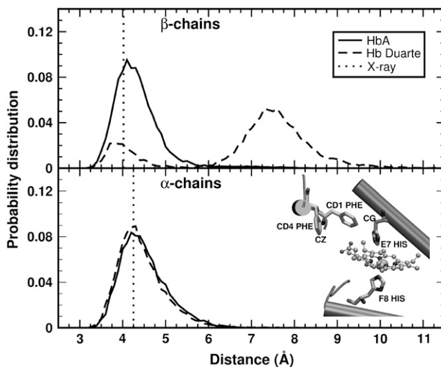
FIGURE 16 Distribution of the distance CZ(PheCD4)-CG(HisE7) (see inset) in the \beta - (upper panel) and \alpha - (lower panel) chains for deoxy HbA (solid lines) and deoxy Hb Duarte (dashed lines) during the simulation. The vertical dotted lines refer to the values extracted from the x-ray structure.
