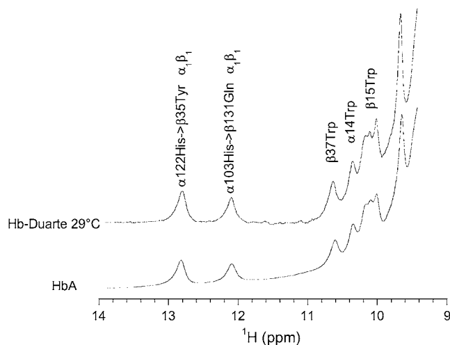
FIGURE 8 Exchangeable proton resonances of HbA and Hb Duarte in the CO form.
