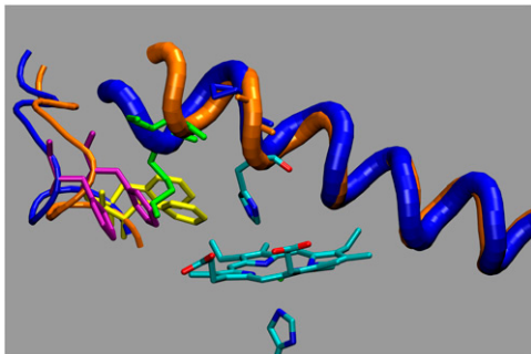
FIGURE 15 Helix section E1–E6 in Hb Duarte (blue tube) and HbA (orange tube), respectively, after 6 and 9 ns of MD simulation.
