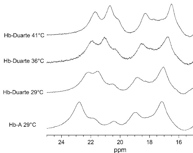
FIGURE 6 Hyperfine shifted proton resonances of HbA and Hb Duarte in the deoxy form collected at several temperatures.
