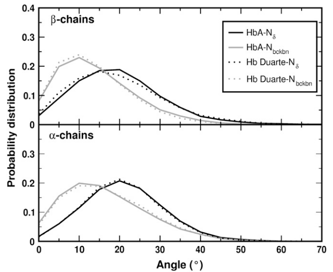
FIGURE 13 Probability distribution of the angles N_{\delta} (His F8)-CO(Leu F4) ( black curves ) and N_{\text{bckbn}} (His F8)-CO(Leu F4) ( gray curves ) for the deoxy Hbs. The solid and dotted curves refer to data for HbA and Hb Duarte, respectively.
