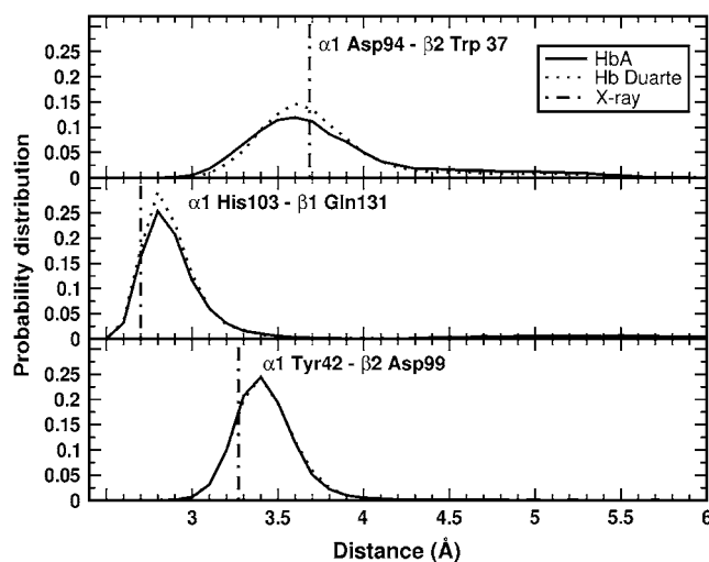
FIGURE 11 Probability distributions of the distances in the switch region of the deoxy Hbs: ( upper panel ) Asp-94–Trp-37 at the \alpha_1\beta_2 interface; ( central panel ) His-103–Gln-131 at the \alpha_1\beta_1 interface; ( lower panel ) Tyr-42–Asp-99 at the \alpha_1\beta_2 interface. Solid and dotted curves are for HbA and Duarte variants, respectively. The dash-dot lines indicate the corresponding distances in the x-ray structures.
