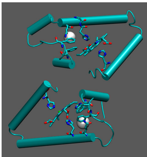
FIGURE 17 Cavity position in hemoglobin (see Table 2). The white spheres refer to the position of the center of mass of the cavities.
