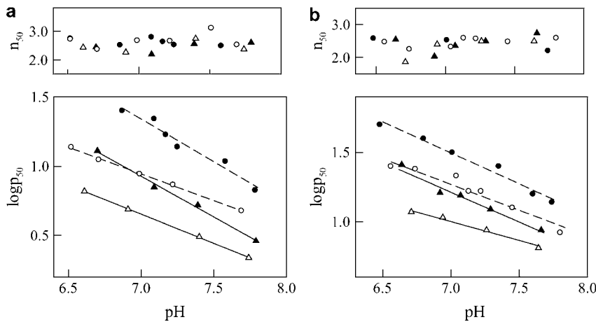
FIGURE 3 Effect of pH on the oxygen affinity ( \log p_{50} ) and cooperativity ( n_{50} ) at (a) 25°C, and (b) 37°C of HbA (circles) and purified Hb Duarte (triangles) in the absence (open symbols) and in the presence (solid symbols) of 5 mM 2,3-DPG. Experimental conditions: 100 mM Bis-Tris/Tris + 100 mM NaCl. O_2 pressure is expressed in torr.
