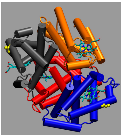
FIGURE 1 Deoxy hemoglobin with the \alpha 1 (red), \alpha 2 (orange), \beta 1 (blue), and \beta 2 (gray) subunits. Heme groups are evidenced via licorice representation, and the substituted ALA residues are in yellow. This figure as well as all the structural figures were obtained with the visualization program VMD (59).
