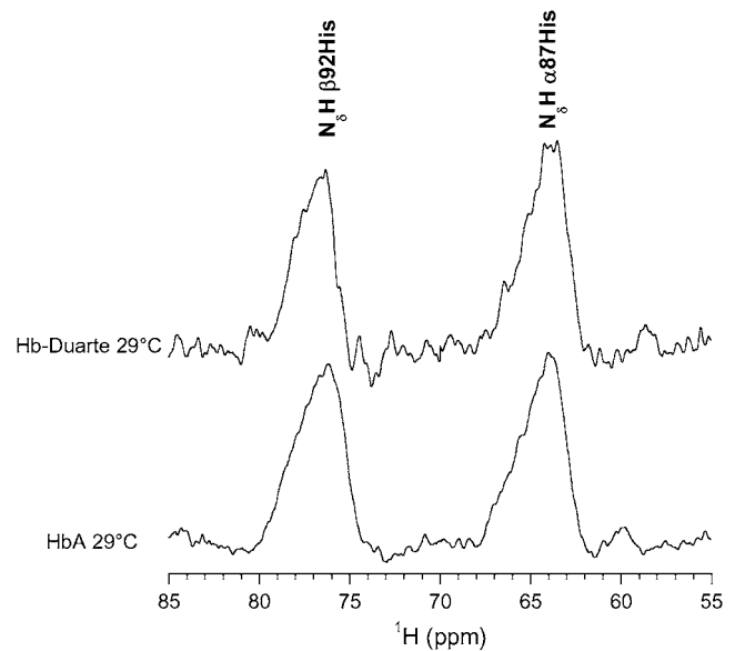
FIGURE 5 Downfield hyperfine-shifted N_{\delta}H of proximal histidines resonances of HbA and Hb Duarte in the deoxy form.
