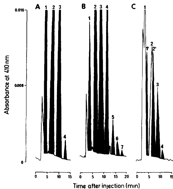
Fig.1. HPLC chromatogram of sulfhydryl group containing material from Cd 2+ exposed plants. (A) G. max , (B) P. aureus (cell culture), (C) L. odoratus . Numbers signify the index n in (\gamma\text{-Glu-Cys})_n\text{-}\beta\text{-Ala} . n = 1, homo-glutathione; n = 2-7, homo-phytochelatins with varying (\gamma\text{-Glu-Cys}) units. Double peaks in C represent: 1 and 1', GSH and h-GSH; 2 and 2', PC 2 and h-PC 2 . Non-metal exposed plants contain neither h-PC nor PC.
