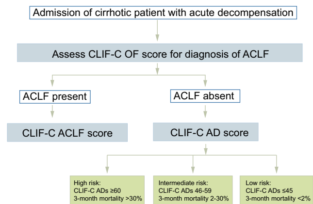
Fig. 4. Algorithm for the sequential use of the EASL-CLIF Consortium predictive scores in patients with cirrhosis admitted to hospital with acute decompensation.
