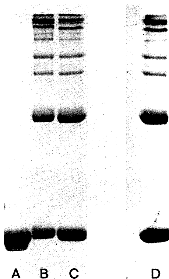
Fig.1. Polyacrylamide slab-gel electrophoresis, in the presence of 0.1% (w/v) SDS, of (A) untreated catalase, (B) catalase crosslinked with 20 mM dimethylsuberimidate, (C) catalase crosslinked with 20 mM [ ^{14}C ]dimethylsuberimidate. The fluorographic detection of radioactivity in track (C) yielded the mirror-image autoradiogram shown in track (D). The observed crosslinking pattern is similar qualitatively with that observed [4], although species greater than the tetramer were unresolved in [4]. The gel presented here clearly resolves higher multimers. The highest order observed, as determined by a plot of log molecular weight against mobility using standard protein markers, is the decamer.
