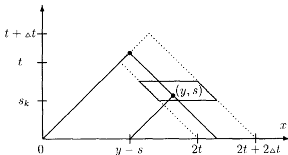
Fig. 1. Computation of \theta'_t .
