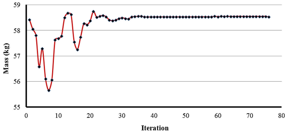
Fig. 6. Change in objective function with respect to iteration.
