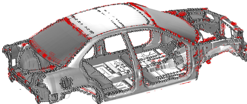
Fig. 5. Vibration FE model of the 1996 Dodge Neon.
