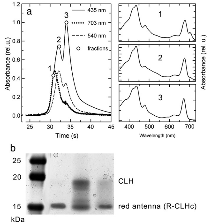
Fig. 3. Results of the gel-filtration of the antenna-containing zone from the sucrose gradient from cells of C. velia grown under incandescent light. (a) Left: elution profiles at wavelengths given in the graph legend; (a) right: absorption spectra of fractions denoted by circles in the left panel; (b) silver-stained SDS-PAGE gel of fractions 1–3.
