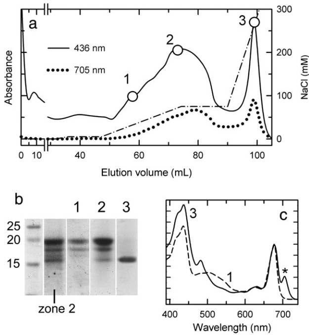
Fig. 2. (a) Results of the anion-exchange chromatography on DEAE Sepharose CL6B of the antenna-containing zone from the sucrose gradient from cells of C. velia . Solid line – absorbance at 436 nm; dotted line – absorbance at 705 nm, dash-dotted line – NaCl concentration (scale on the right side of the graphs); (b) Coomassie-stained SDS-PAGE gel of the fractions; (c) absorption spectra of fractions 1 (solid line) and 3 (dashed line) denoted by circles in the left panel. Spectra of the intermediate fraction 2 corresponded to a linear combination of spectra 1 and 2, in agreement with (b) hence were omitted for clarity. The asterisk highlights the red-shifted absorption band of fraction 3.
