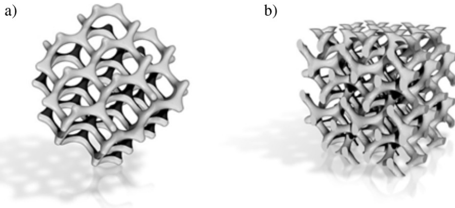
Fig. 7. (a) The single gyroid morphology with I4_132 symmetry, (b) the double gyroid morphology with Ia\bar{3}d symmetry. Adapted with permission from Ref. [116].
