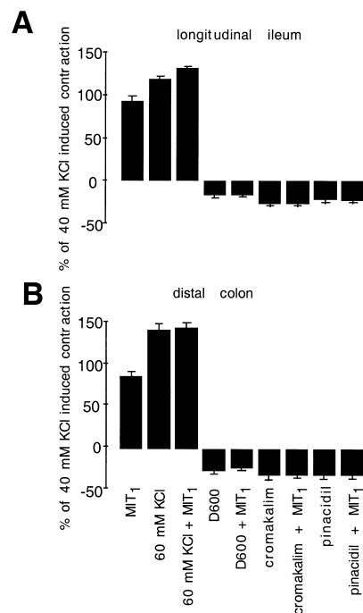
Fig. 4. Effect of the L-type voltage-dependent Ca 2+ channel antagonist D600 (10 \mu M), the K + channel openers cromakalim (10 \mu M) and pinacidil (10 \mu M) and increased external K + concentration (60 mM) on the contraction induced by (1 nM) MIT 1 on guinea-pig longitudinal ileum muscle (A) and guinea-pig distal colon (B). Each condition is expressed as a percentage of the maintained contraction induced by 40 mM K + . Results are expressed as mean values of four to eight experiments.
