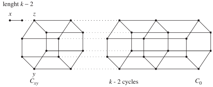
Fig. 4. The gadget from [8] replacing an edge (x, y) , C_0 is common to all the edges.
