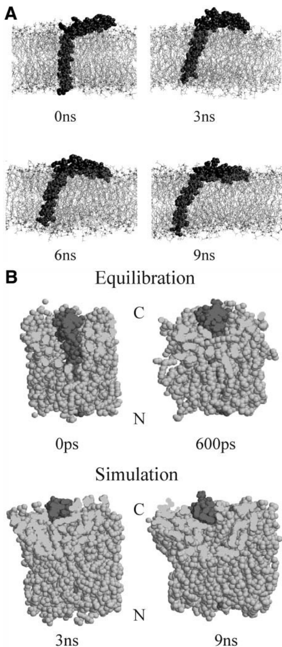
FIGURE 1 Snapshots of the protein ( black ) embedded in a lipid bilayer ( thin gray chains , gray spheres represent the phosphorous headgroups) at 0, 3, 6, and 9 ns ( A ). View from the C- to the N-terminal end of Vpu along the axis of helix-2 ( dark ) lying on top of the bilayer ( gray ) before (0 ps) and after 600 ps of equilibration with the protein ( dark ) restraint ( B ). Snapshots taken from the simulations at 3 ns and 0 ns are shown in the lower half. The figures are created with the software Rasmol in the slab mode showing the atoms with their van der Waals radii. Plain gray spots are sliced atoms due to the slab-mode representation.
