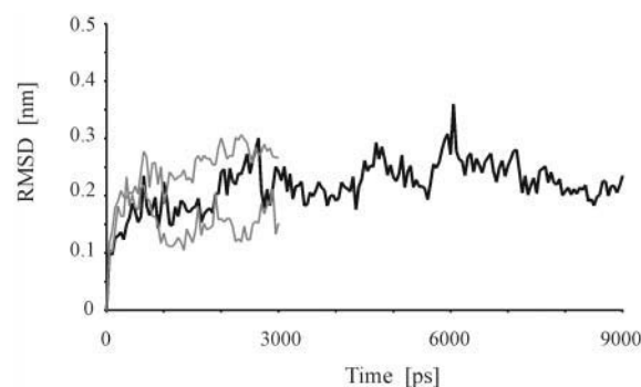
FIGURE 2 Root mean square deviation (RMSD) of the \alpha -atoms of the simulation over 9 ns ( black trace , thick line ) and two simulations each over 3 ns ( gray and black thin lines ).
