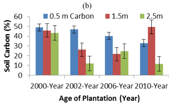
Fig. 1. (a) Soil carbon variation with age of plantation and soil depth (Wet season)- with error bars; (b) Soil carbon variation with age of plantation and soil depth (Dry season)
