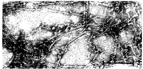
Fig.3. Electron micrograph of yeast actin-like protein sample negatively stained with 1% uranyl acetate; bar = 100 nm.
