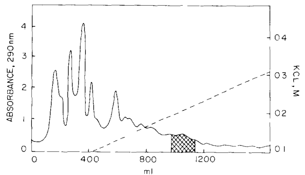
Fig 1 DEAE-cellulose chromatography of Saccharomyces cerevisiae extract. Extract 150 ml was applied to a DEAE-cellulose column (Whatman DE 52, column size 50 × 2.5 cm). Column was pre-equilibrated with buffer II (10 mM imidazole, 0.1 mM CaCl_2 , 0.5 mM ATP, 0.2 mM DTT, pH 7.5) containing 0.1 M KCl and saturated with ATP [7]. After application of sample, the column was washed with 200 ml buffer II containing 0.1 M KCl and elution was carried out using 2 l linear 0.1–0.5 M KCl gradient on buffer II at 50 ml/h flow rate. The elution of protein was monitored by measurement of A_{290\text{ nm}} to decrease ATP interference during measurements. All chromatography steps were done at 4°C. Hatched area corresponds to the fractions where actin-like protein was found as judged by the inhibition of DNase I
