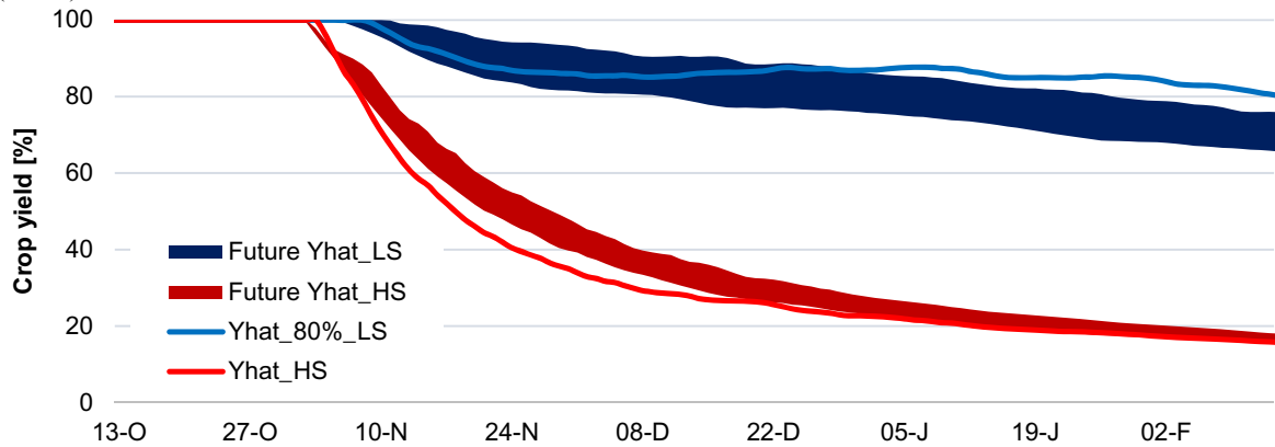
Fig. 5. Relative crop yield Y_{LS}^{80\%} (blue line) and \hat{Y}_{HS} achieved for the irrigation quantity W_{LS}^{80\%} (red line) for current conditions. Blue and red surfaces depict the range of future \hat{Y}_{LS} and \hat{Y}_{HS} for the same amount of irrigation ( W_{LS}^{80\%} ).
