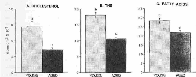
Figure 3. Lipid Synthesis Is Abnormal in Aged Murine Epidermis in Vitro . Full thickness skin samples from young and aged mice were incubated with [ 14 C]acetate for 3 h, and the lipids were extracted, saponified, and fractionated as described in the text. ( a vs. a , b vs. b ; p < 0.05 contrast c vs. c ; p < 0.1). n = 3; mean ± SEM.
