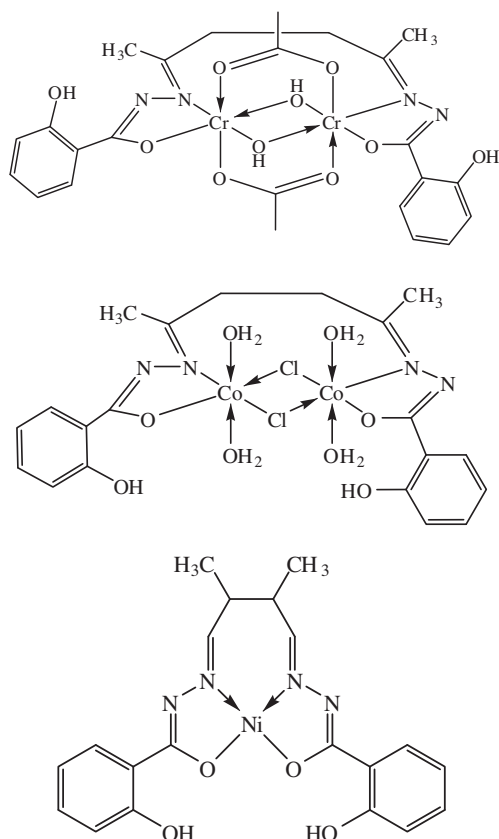
Scheme 3 Structures of [\text{Cr}_2(\text{H}_2\text{L})(\text{OAc})_2(\text{OH})_2] \cdot 2\text{H}_2\text{O} , [\text{Co}_2(\text{H}_2\text{L}_1)(\text{H}_2\text{O})_4\text{Cl}_2] \cdot 2\text{H}_2\text{O} and [\text{Ni}(\text{H}_2\text{L})] \cdot 3\text{H}_2\text{O} .
