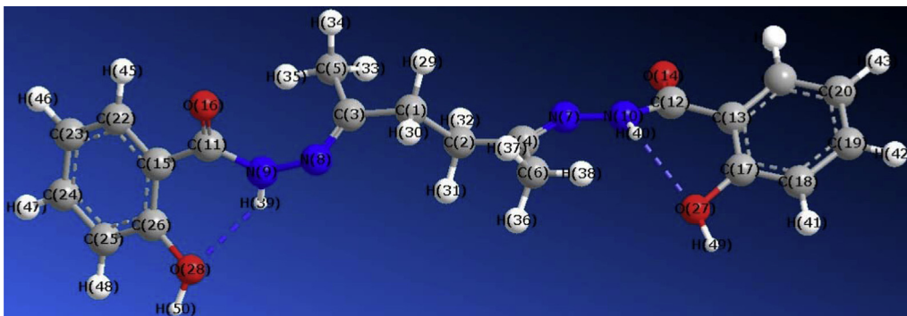
Scheme 1 Molecular modeling of \text{H}_4\text{L} using HyperChem 7.5 program optimized using molecular mechanics (MM+) at PM3 using the Polak-Ribiere algorithm.
