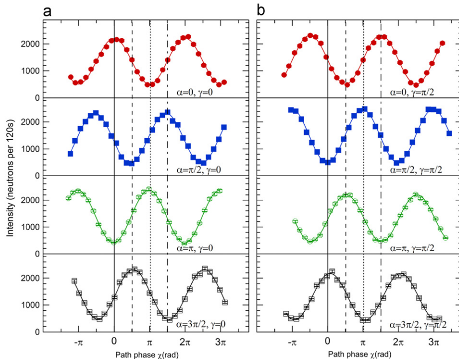
Fig. 3. Typical intensity modulations obtained by varying the path phase \chi . The energy phase \gamma is tuned at (a) 0 and (b) \pi/2 . The spin phase \alpha is set at 0, \pi/2, \pi , and 3\pi/2 (from upper to lower panels).
