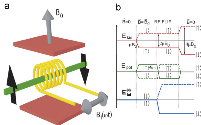
Fig. 1. Coherent energy manipulation scheme by the interaction with an oscillating magnetic field. (A) Spin-flip process through the time-dependent magnetic field, B_1(\omega t) . (B) Energy diagram, i.e., kinetic, potential, and total energies, of neutrons in passing through the magnetic field configuration of a RF-flipper.
