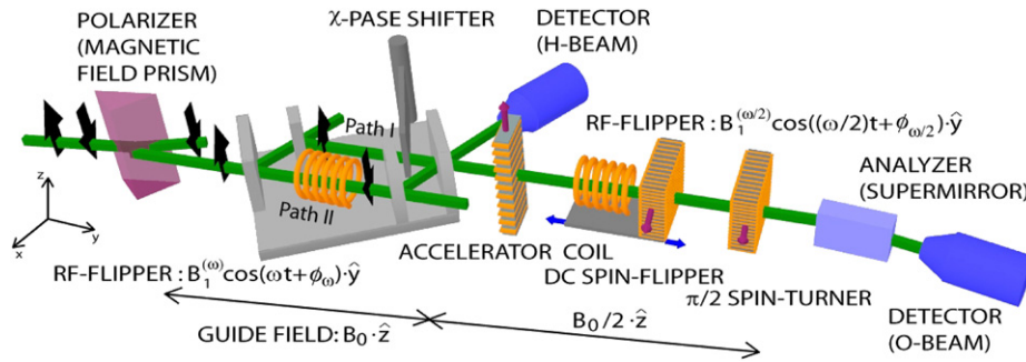
Fig. 2. Experimental setup for the study of tripartite entangled GHZ-like state in a single-neutron system.
