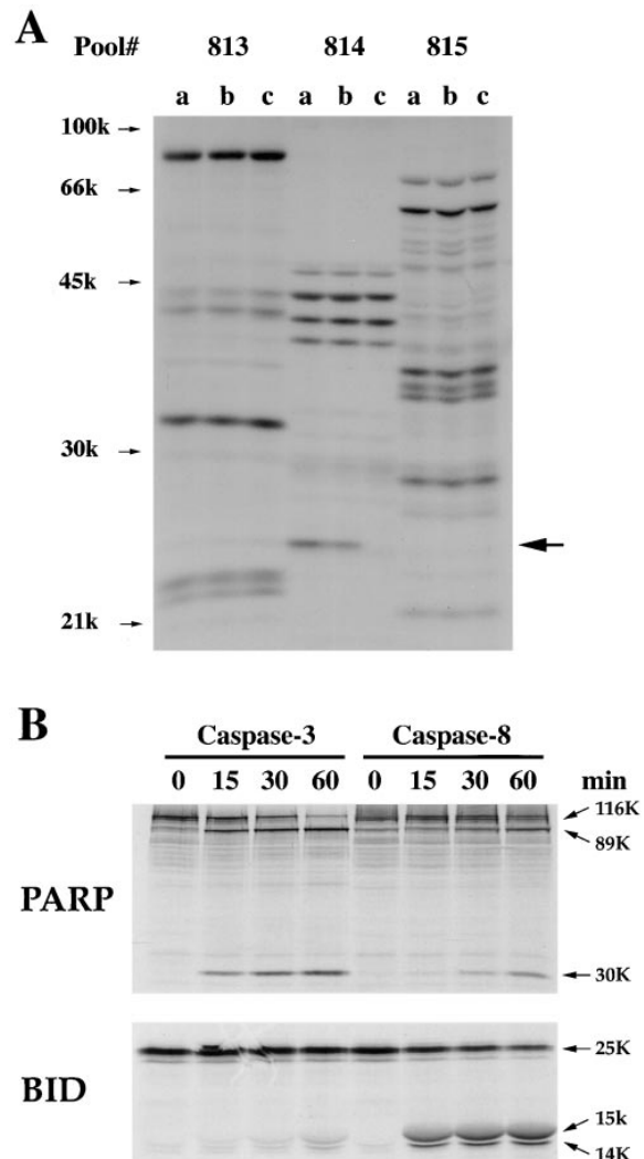
Figure 1. BID Is a Preferred Substrate of Caspase 8 In Vitro (A) Primary screening of caspase substrates by small pool in vitro expression cloning. Different pools of 35 S-labeled proteins were incubated with bacterial lysates containing either no caspase (a), Casp2 (b), or Casp8 (c) for 2 hr at 37°C. The reactions were terminated and analyzed by 12% SDS-PAGE. An arrow points to a band, later identified as murine BID, that disappeared in the presence of Casp8. (B) BID is a better substrate of Casp8 than of Casp3. 35 S-labeled N-terminal T7-tagged BID was incubated with either Casp3 or Casp8 for indicated time periods, and the cleavage products were analyzed by 15% SDS-PAGE.
