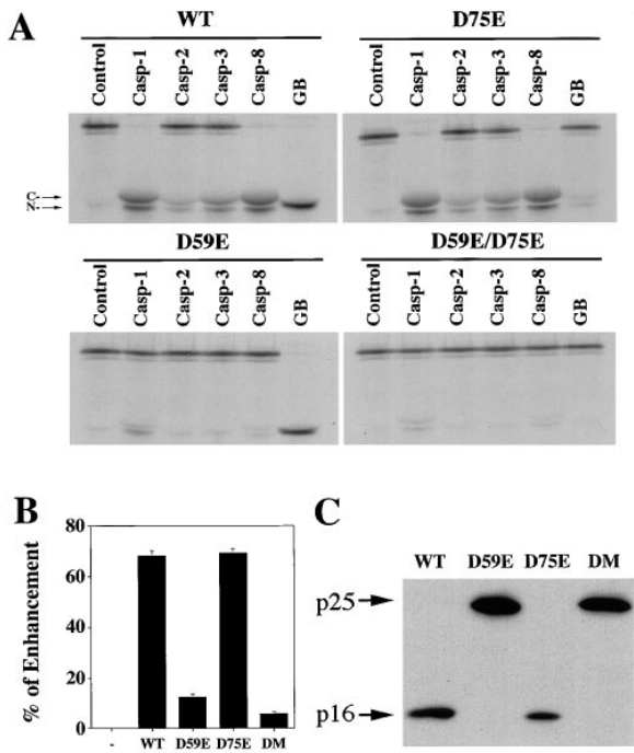
Figure 3. Proapoptotic Activity of BID Strongly Depends upon Its Cleavage
