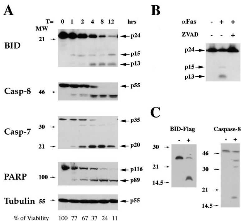
Figure 2. BID Is Cleaved In Vivo during Fas- and TNF \alpha -Induced Apoptosis
