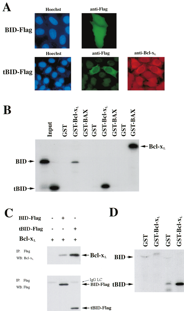
Figure 5. Truncated BID Has a Stronger Affinity for Bcl x L than Its Precursor
