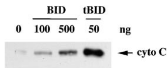
Figure 7. Truncated BID Induced the Release of Cytochrome c from Partially Purified Mitochondria In Vitro
