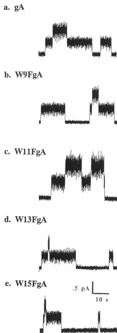
FIGURE 2 Current traces in 1-M formamidineum with gA, W9F gA, W11F gA, W13F gA, and W15F gA in GMO ester/hexadecane membranes at 50 mV. Sampling frequency 200/s, cutoff frequency 60 Hz. Room temperature (22–24°C).
