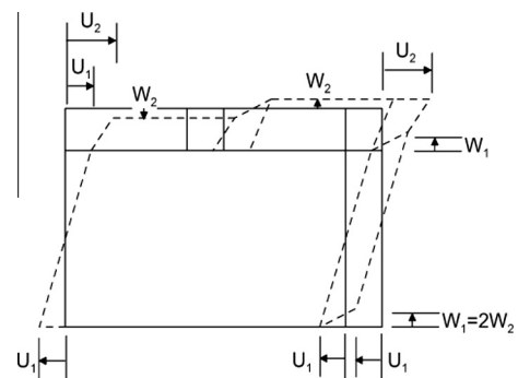
Fig. 4. Strain-periodic kinematically admissible microscopic strain field under in-plane macroscopic shear.
