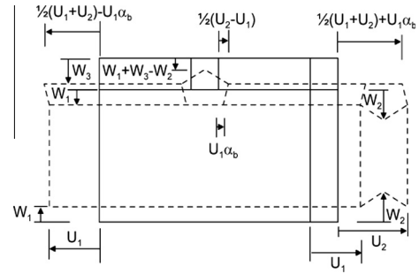
Fig. 3. Strain-periodic kinematically admissible microscopic strain field under horizontal or vertical macroscopic stresses.
