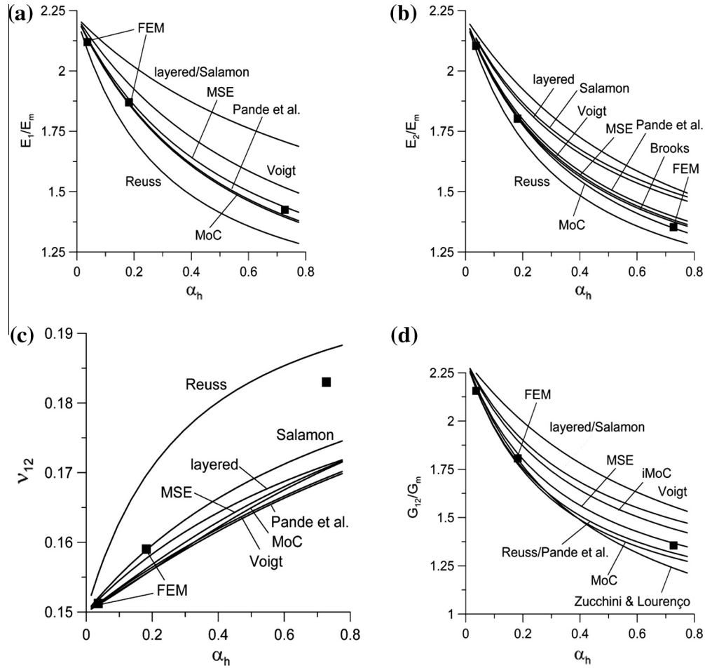
Fig. 6. Header bond brickwork: predicted values of the macroscopic in-plane elastic constants vs. bed joint thickness-to-brick height ratio. (a) E_1 , (b) E_2 , (c) v_{12} , and (d) G_{12} .
