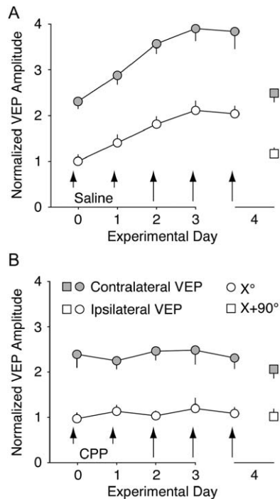
Figure 6. NMDA Receptor Dependence
