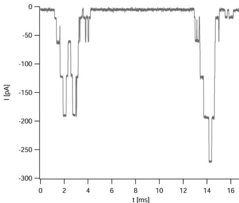
FIGURE 4 Single channel recordings from alamethicin in a lipid bilayer. Alamethicin was given to the electrolyte solution (1 M NaCl) from a methanol stock solution. Apertures in the chips used for bilayers recordings had diameters of 10 \mu\text{m} . A potential of 100 mV was applied and the recording was low-pass filtered at 10 kHz.
