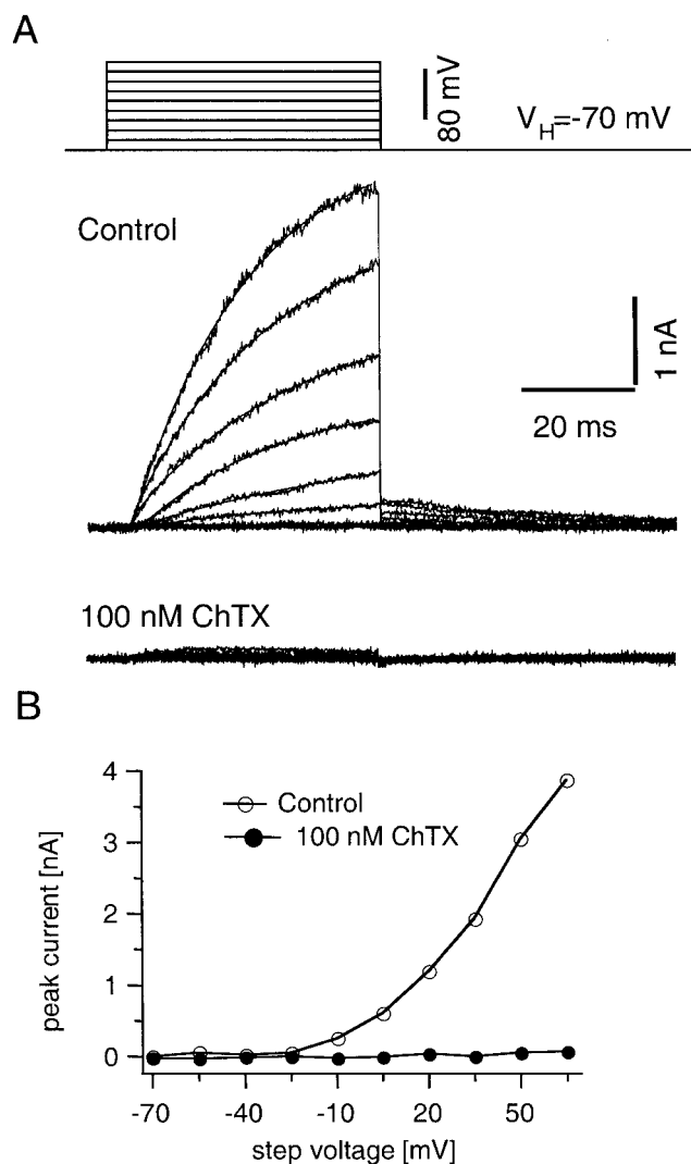
FIGURE 3 Pharmacological characterization of K-channels using the chip device. (A) CHO cells overexpressing a BK-type \text{Ca}^{2+} -activated potassium channel were recorded. Outward currents were blocked by the selective blocker charybdotoxin (100 nM). (B) Current-voltage relations from the experiment shown in A.
