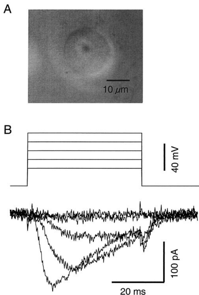
FIGURE 2 Whole cell \text{Ca}^{2+} -currents from a neuroblastoma cell recorded with the chip device. (A) Video-micrograph of a N1E115 neuroblastoma cell positioned on top of the quartz chip device. The aperture is discernible below the cell. (B) \text{Ca}^{2+} -currents were elicited in response to voltage steps from a holding potential of -70 mV.
