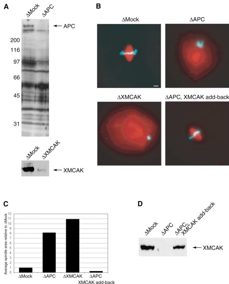
Figure 1. The Large Spindle Structures Formed in Egg Extracts Depleted of APC by a Combination of Carboxyl- and Amino-Terminal Antibodies Are Similar to Those Formed in XMCAK-Depleted Extracts
