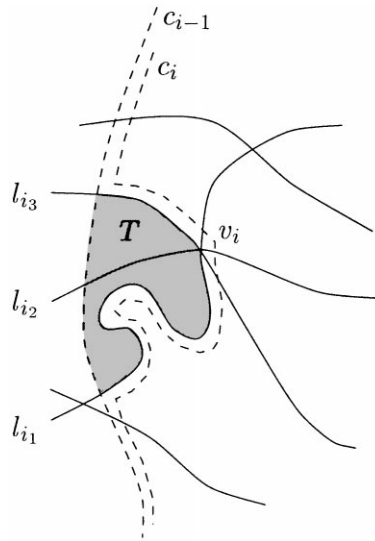
Fig. 4. Defining c_i based on c_{i-1} and the shaded triangular region T .
