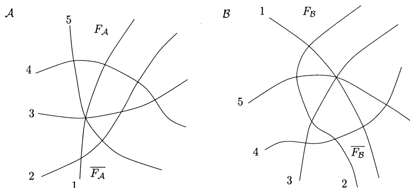
Fig. 1. Arrangements \mathcal{A} and \mathcal{B} are isomorphic as arrangements but non-isomorphic as marked arrangements.
