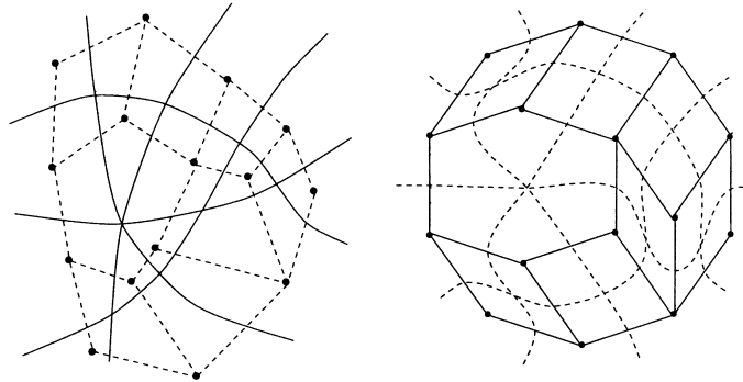
Fig. 6. An arrangement with its dual graph and the dual graph as zonotopal tiling.
