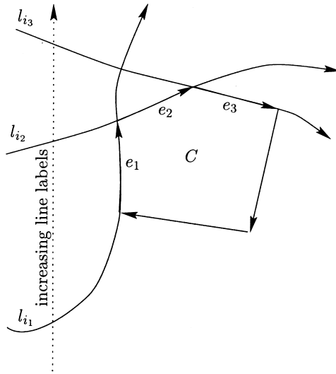
Fig. 3. Assuming an oriented cycle.
