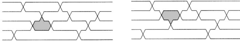
Fig. 7. Elementary flip at the shaded triangle.
