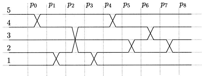
Fig. 5. A wiring diagram for the arrangement of Fig. 2.
