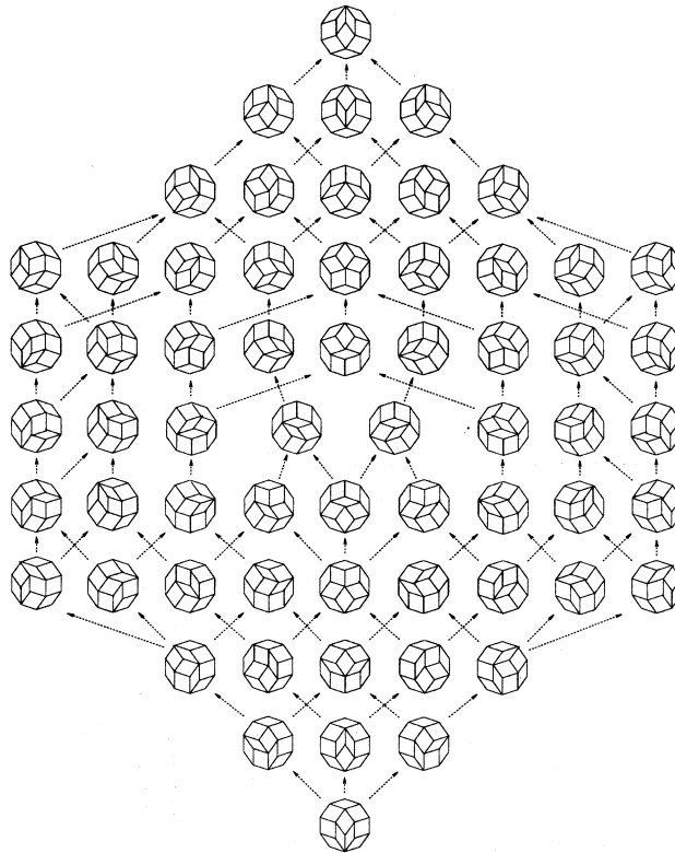
Fig. 8. The graph \mathcal{G}_5 as diagram of the signotope order S_3(n) .
