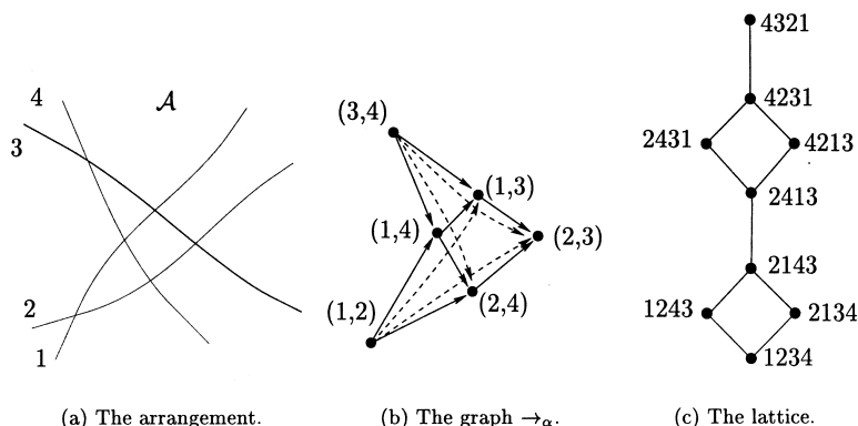
Fig. 9. Illustrations for Example B.
