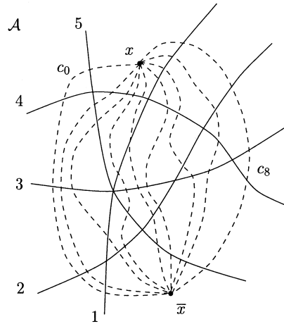
Fig. 2. A sweep for arrangement \mathcal{A} .
