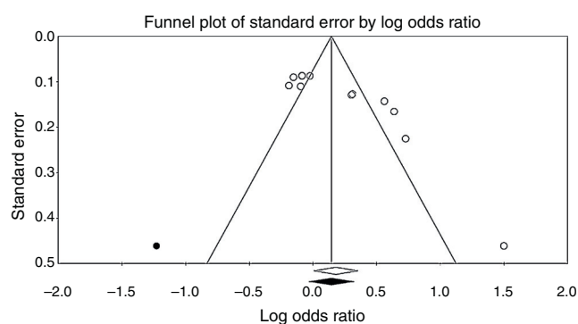
Figure 3 Funnel plot assessing publication bias.
