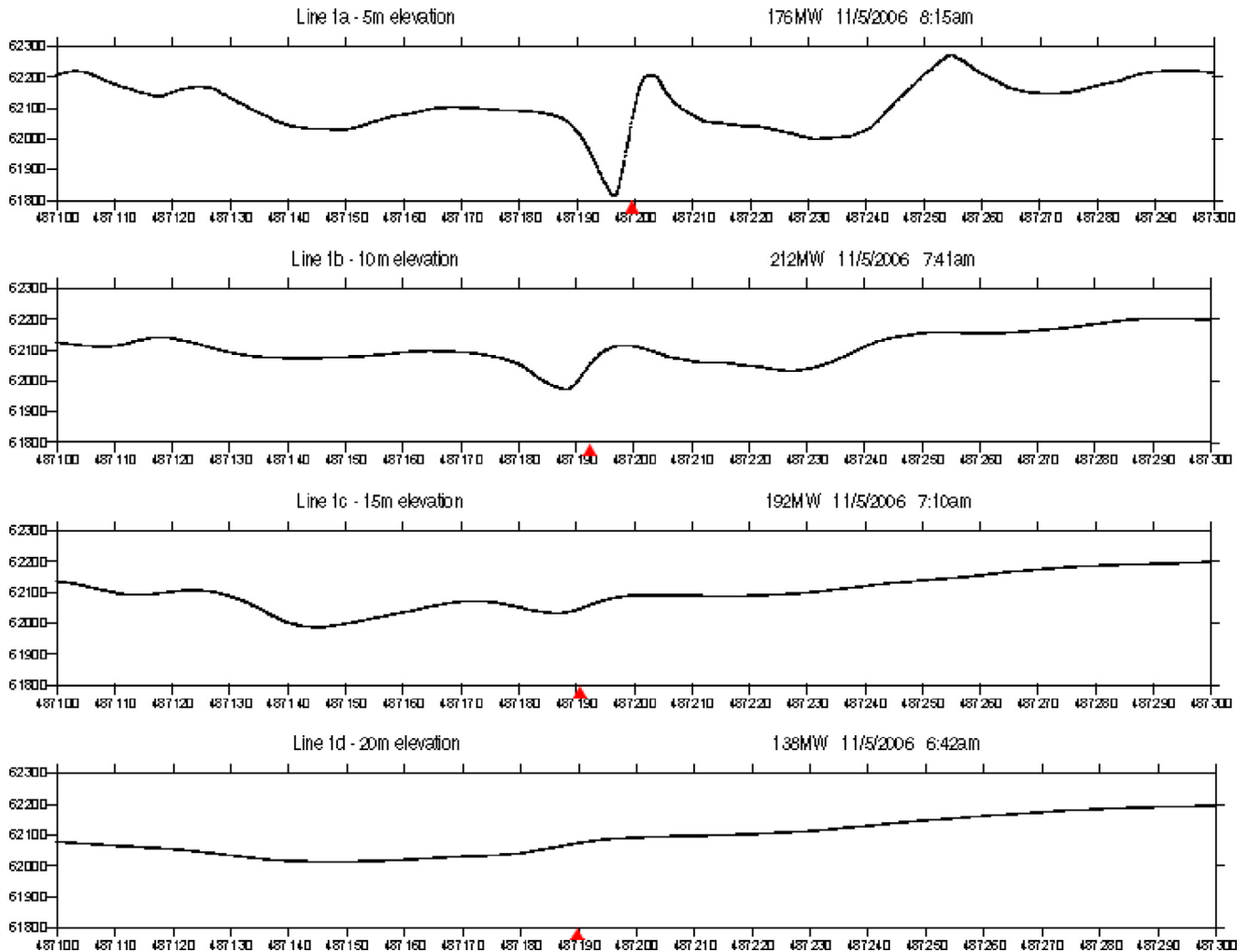
Fig. 7. Magnetic profiles for one of three crossing sets. Red triangles mark the inferred cable position of each transect. Y axis is magnetic field strength in units of nanoTeslas (nT), x-axis is Eastings (metres). The time and cable power for each transect is also shown.
