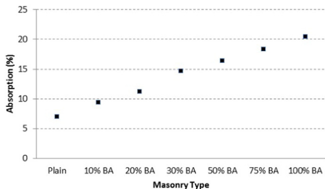
Fig. 5. Water absorption results.
