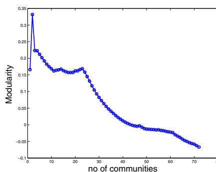
Figure 5: Modularity Score
