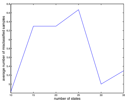
Figure 4: Selection of Number of States
