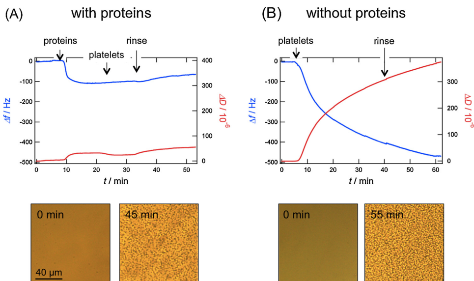
Fig. 3. QCM-D frequency and dissipation versus time curves (upper panels) and light microscopy (lower panels) of platelets adhering on \text{TiO}_2 coated surface in (A) a protein-rich environment and (B) a protein-poor environment. Light microscopy images were taken during the QCM-D experiment, before injection of platelets and in the end of the experiment.
