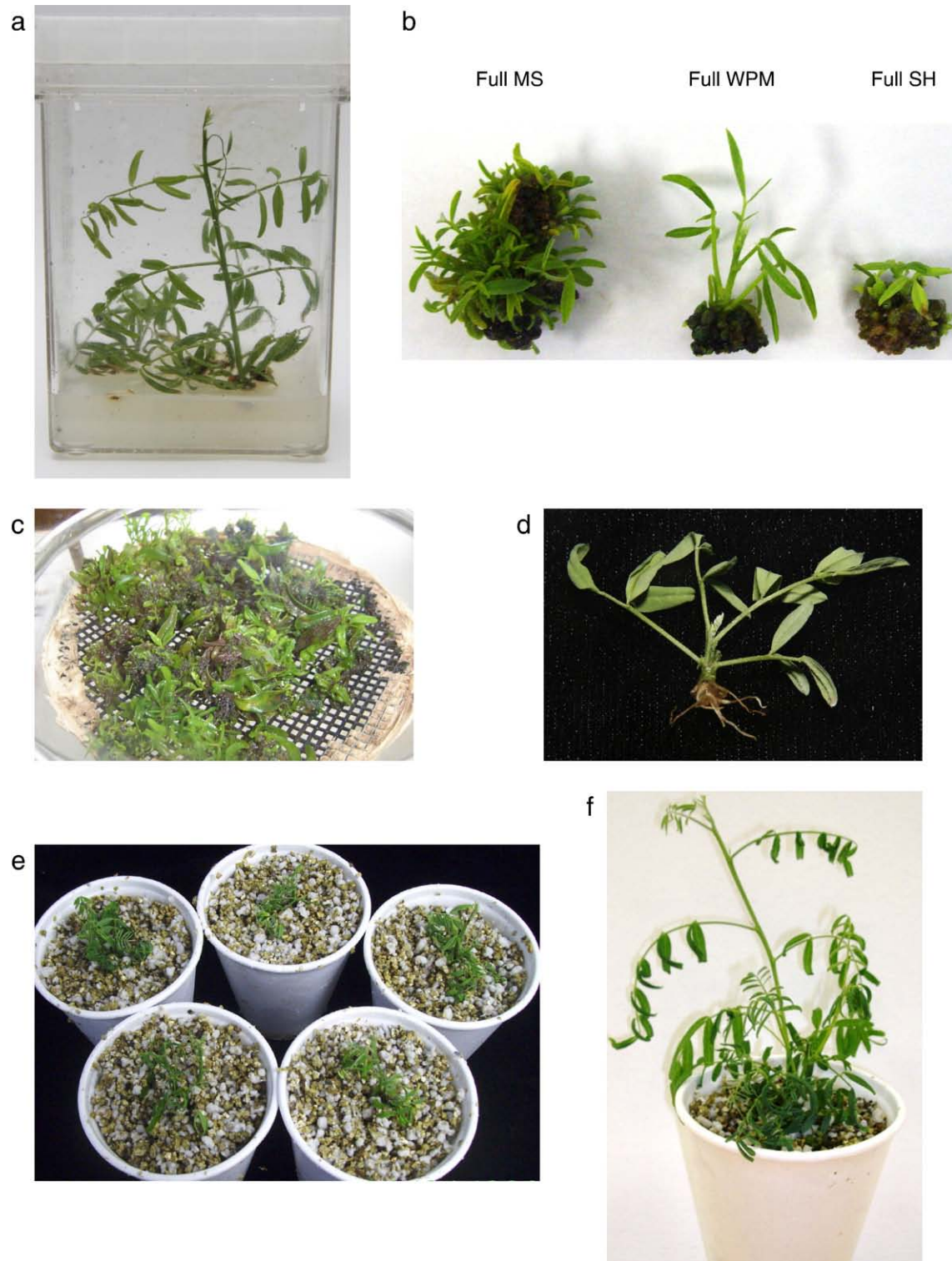
Fig. 1. In vitro shoot multiplication, rooting and acclimatization of Lessertia frutescens : (a) shoot multiplication on MS supplemented with BA (2.22 \mu\text{M} ) and NAA (0.54 \mu\text{M} ) after 6 weeks in culture; (b) shoot multiplication in different media after 6 weeks in culture; (c) shoot multiplication in temporary immersion bioreactor showing symptoms of hyperhydricity after 6 weeks in culture; (d) in vitro rooting after 4 weeks in culture; (e) plantlets at day zero of acclimatization; (f) acclimatized plant.
