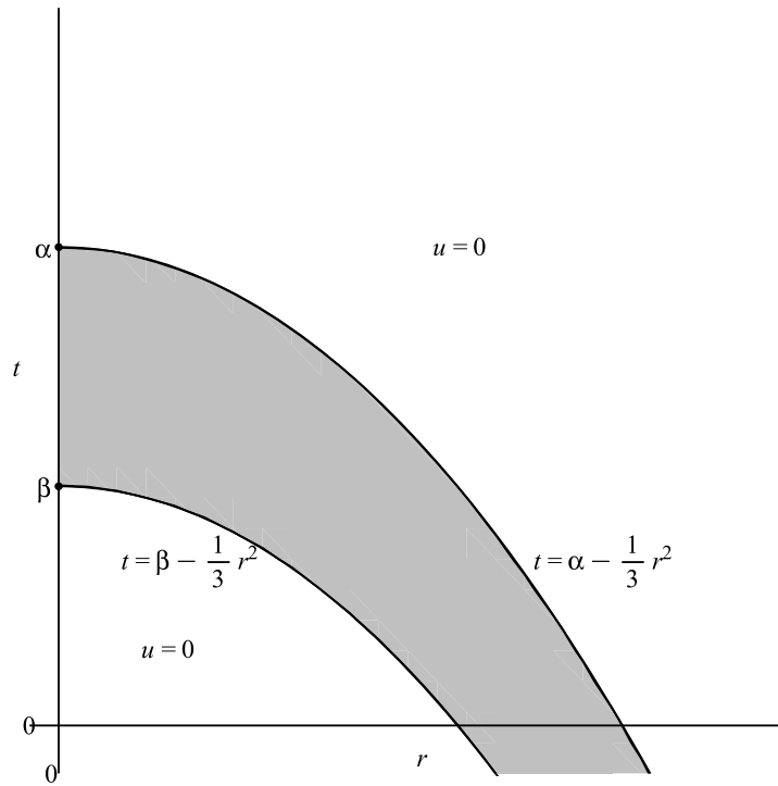
Fig. 5. Space-time graph of solution (89).
