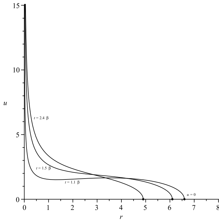
Fig. 6. Graph of solution (89) with \beta = 5 , \alpha = 20 .
