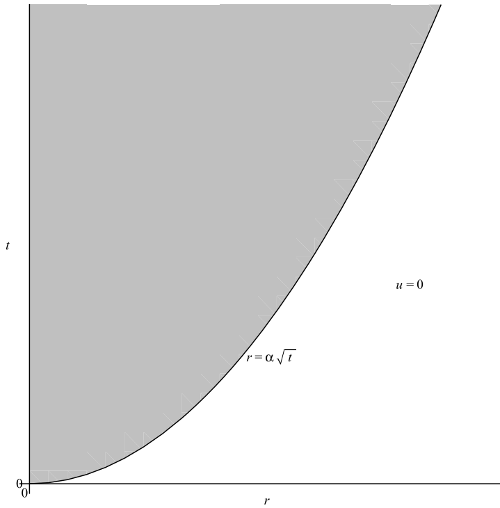
Fig. 1. Space-time graph for solution (67).
