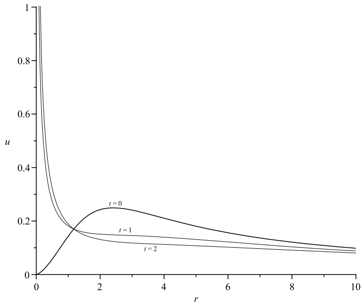
Fig. 4. Graph of solution (54).
