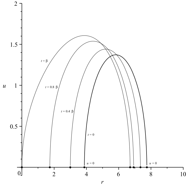
Fig. 7. Graph of solution (89) with \beta = 5 .
