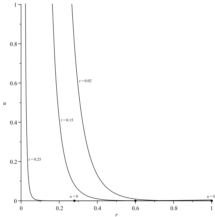
Fig. 2. Graph of solution (67) with n = 6 ( q + 1 = 1/2 ).
