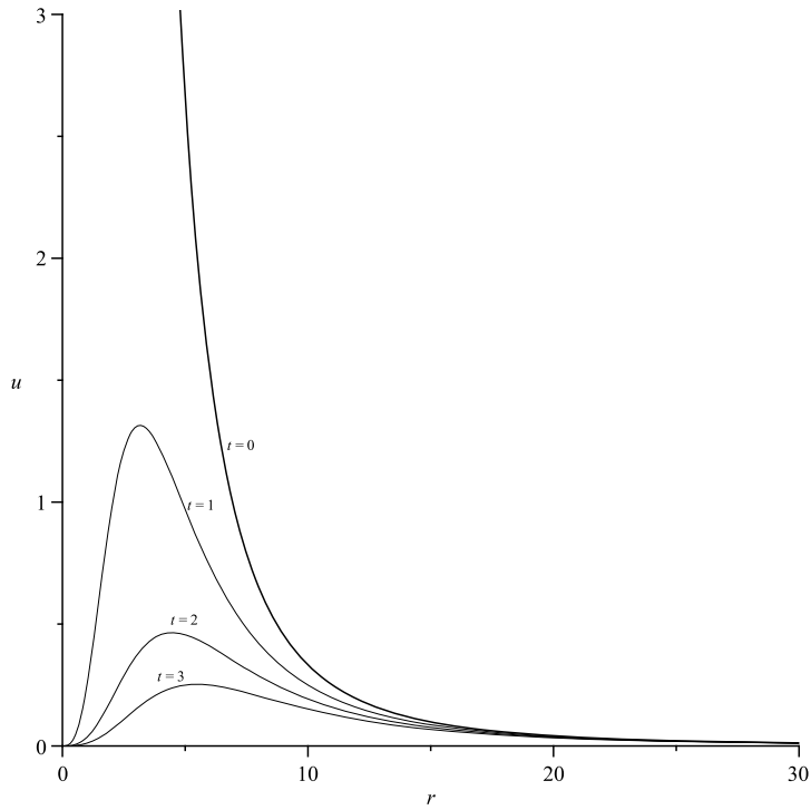
Fig. 3. Graph of solution (84) with \nu = 3 .
