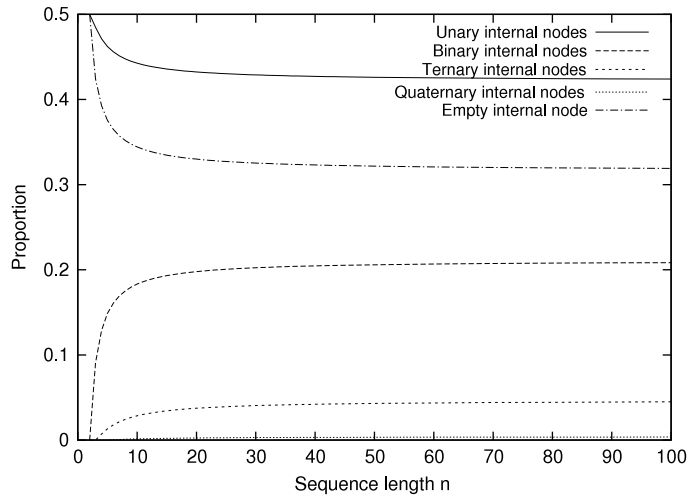
Fig. 8. Evolution of the node degree distribution for trees of increasing size in the uniform model. The asymptotic proportions of nodes of degree (0, 1, 2, 3, 4) are respectively (81/256, 27/64, 27/128, 3/64, 1/256).
