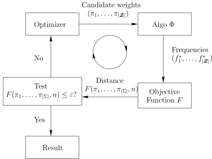
Fig. 7. General principle of our heuristic approach to the problem of computing weights \pi that achieve targeted frequencies \mu .
