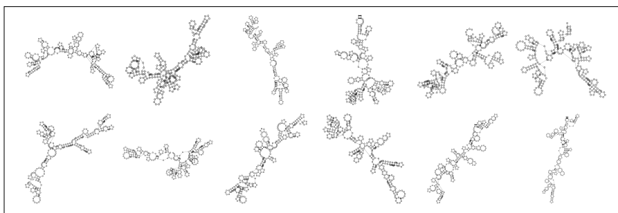
Uniform model \mathcal{M}_0
