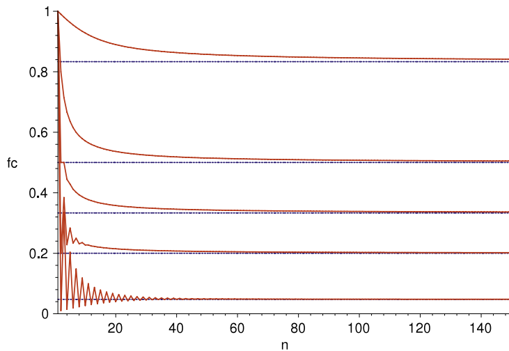
Fig. 2. Convergence toward the asymptotic regimes (Dashed lines) of the proportions f_c (Solid lines) of unary nodes among \pi -weighted unary/binary trees of size n . Five values for the couple (\pi, f_c) are shown here (From top to bottom): (10, 5/6) , (2, 1/2) , (1, 1/3) , (1/2, 1/5) , and (1/10, 1/21) .
