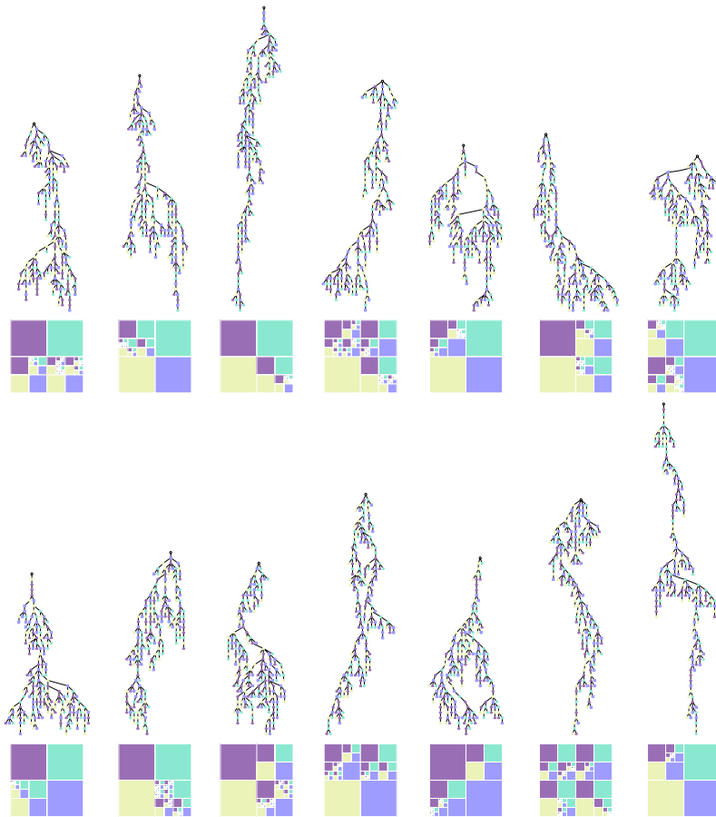
Uniformly generated quad trees
