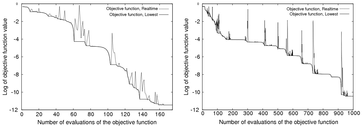
Fig. 12. Minimization of the objective functions in the Helices (Left) and Loops (Right) models. A logarithmic scale is used for the value of the objective function (Y-axis).
