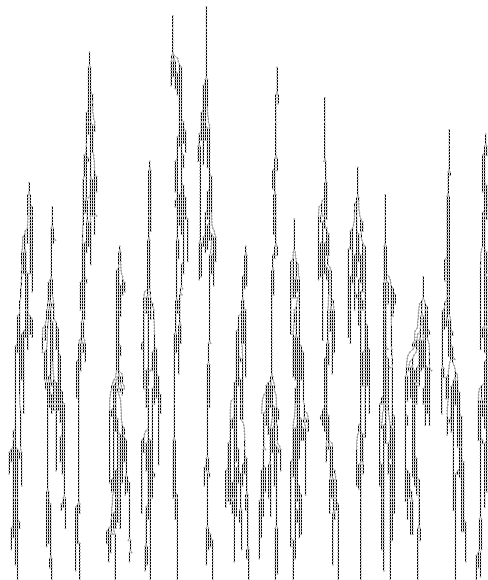
Fig. 3. Unary-binary trees associated with weighted Motzkin words of size 500, for different values of \pi the weight of unary nodes.
