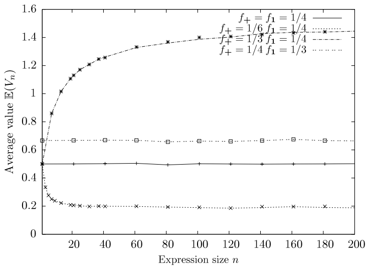
Fig. 4. Average value of an arithmetic expression, computed by generating 100 000 random expression, for various sizes n and frequencies of symbols + and 1 .
