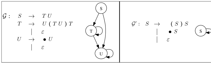
Fig. 1. Two equivalent grammars for the Motzkin language along with their dependency graphs.
