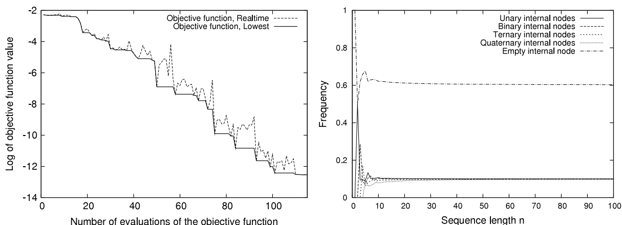
Fig. 9. Left: Weight optimization for weighted quadtrees of size 201. The targeted proportions are 121/201 (resp. 20/201) for nodes of degree 0 (resp. 1, 2, 3 and 4). Right: Node degree distributions for weighted quad trees of increasing size in our weighted model. Although formally the computed weights only work for size 201 structures, a good approximation of the targeted distribution is already observed for smaller sizes.
