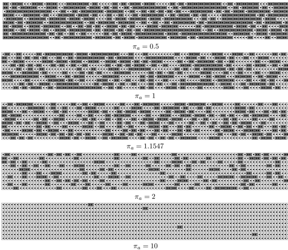
Fig. 5. Sets of randomly generated Fibonacci words of length 100 for different values of \pi_a . White boxes: a 's; grey boxes: b 's.
