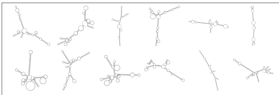
Loops model \mathcal{M}_L : Constrained hairpins and multiple loops.
