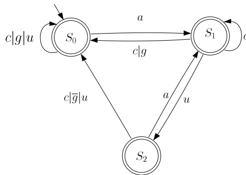
Fig. 6. A finite state automaton recognizing the language generated by the grammar.
