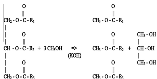
Figure 1 Transesterification reaction.
