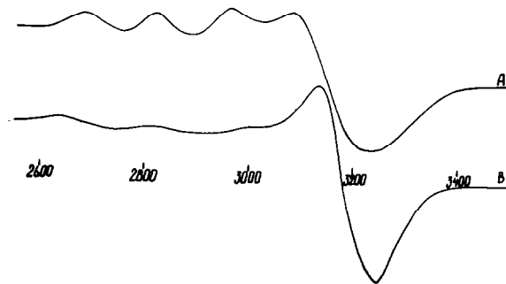
Fig. 4. EPR-spectra of native (A) and H_2O_2 -inactivated (B) dismutases. The native protein sample was in 0.025 M phosphate buffer, pH. 7.0. Inactivation was carried out by addition of 0.2 ml 10% H_2O_2 to 1 ml dismutase solution. After 10 min incubation at room temp. the EPR-spectrum was recorded. The recording conditions were the same as those for the case shown in fig. 2 with the exception of receiver gain being 1.6 \times 10^2 . EPR-spectral parameters of native dismutase: A_{\parallel} = 140\text{G} ; g_{\parallel} = 2.26\text{g} ; g_{\perp} = 2.07\text{g} . EPR-spectral parameters of inactivated dismutase: A_{\parallel} = 172\text{G} ; g_{\parallel} = 2.25\text{g} ; g_{\perp} = 2.04\text{g} .
