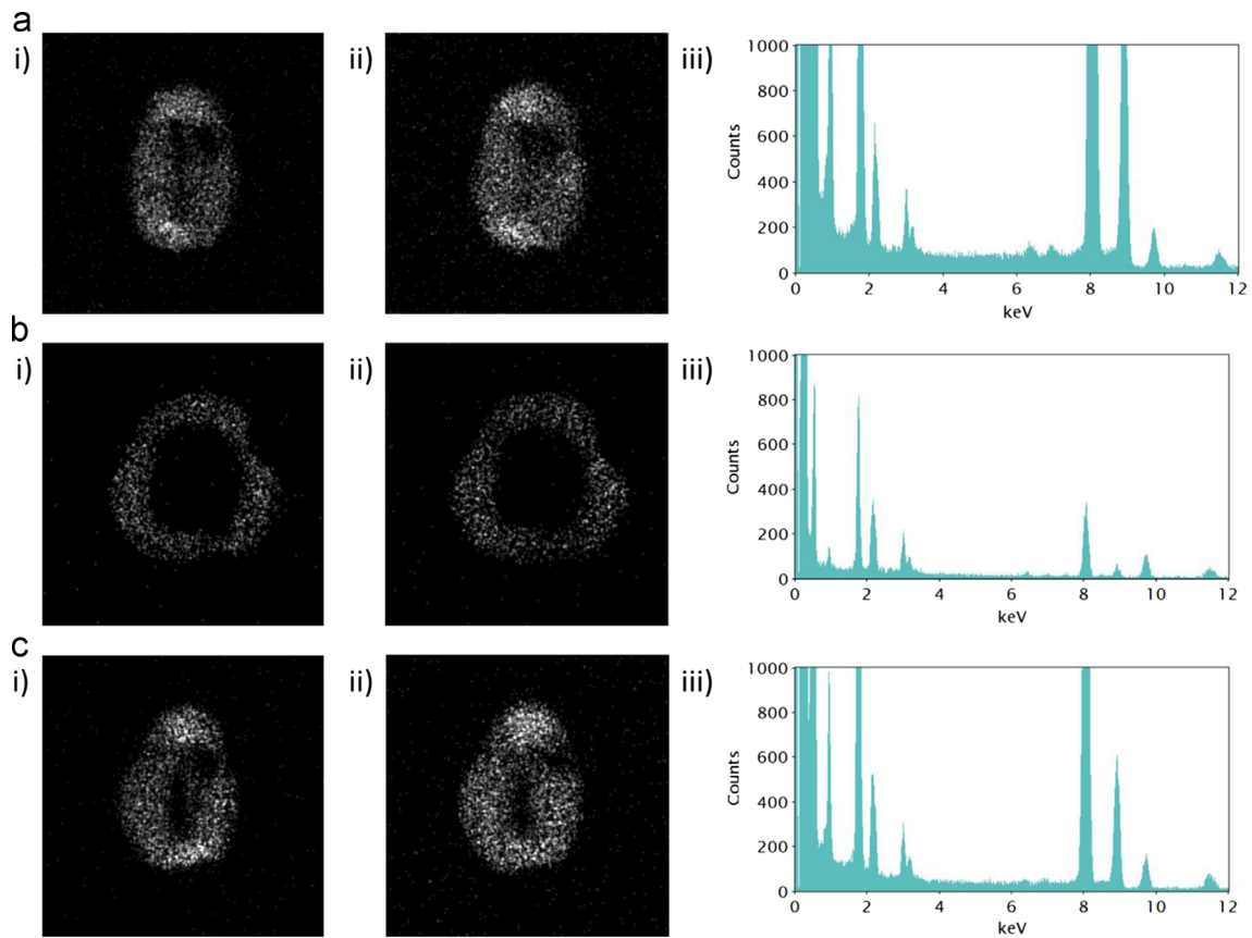
Fig. 10. Projections at (a) -60^\circ , (b) 0^\circ and (c) 60^\circ for (i) Au L \alpha counts and (ii) Ag L \alpha counts. (iii) Spectra from the full spectrum images at (a) -60^\circ , (b) 0^\circ and (c) 60^\circ .
