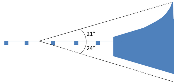
Fig. 4. Schematic diagram showing the elevation angles from the sample at which the holder and grid bars will shadow emitted X-rays above and below the specimen in the direction of a single Super-X detector (45° azimuthal angle).
