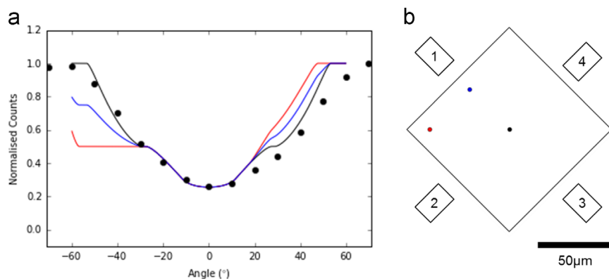
Fig. 5. Modelling detector shadowing using the model of Yeoh et al. [22]. (a) Plot of normalised counts with respect to tilt angle for the positions within a grid square indicated in (b). Experimental data points for Au L\alpha (9.7 keV) X-rays (reproduced from Fig. 2c) are also shown (black dots) for reference. (b) Diagram indicating nanoparticle position within a 90\ \mu\text{m} \times 90\ \mu\text{m} grid square with black in the centre, blue 10\ \mu\text{m} from the edge towards detector 1 and 45\ \mu\text{m} from the edge towards detector 2 and red 10\ \mu\text{m} from both edges towards detector 1 and detector 2. (For interpretation of the references to color in this figure legend, the reader is referred to the web version of this article.).
