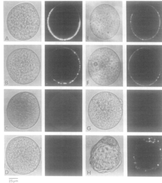
Figure 2. Indirect Immunofluorescence of Integrins on the Surface of Unfertilized Mouse Eggs
