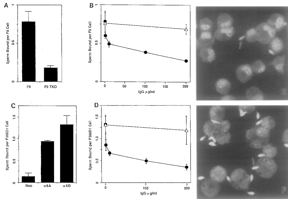
Figure 5. Sperm Binding to Cultured Cells
