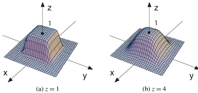
Fig. 6. Graphs of the approximation (25) of the solution of problem (P 3 ) for two different values of z and ε = 0.1.
