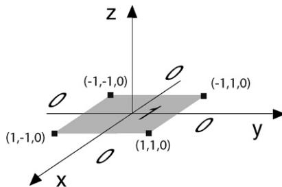
Fig. 5. Domain \Omega_3 and boundary condition of problem (P 3 ).
