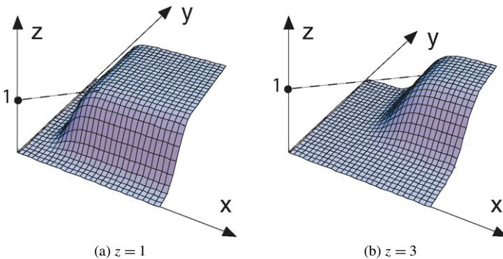
Fig. 4. Graphs of the approximation (22) for the solution of problem (P' 2 ) with \epsilon = 0.1, \vec{v} = (1, 1, 1)/\sqrt{3} and two different values of z .
