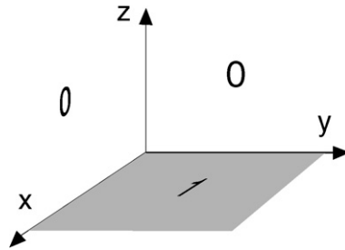
Fig. 3. Domain \Omega_2 = (0, \infty) \times (0, \infty) \times (0, \infty) and boundary conditions of problem (P_2) .
